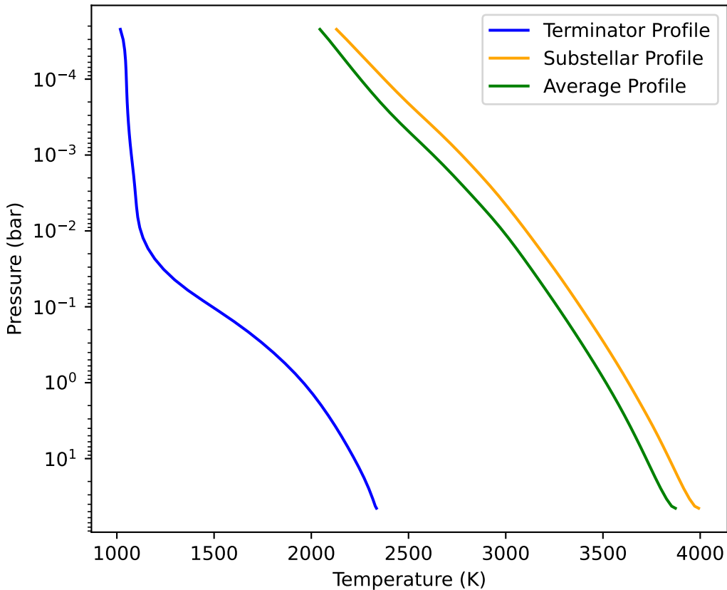
PT Profile TOI561
