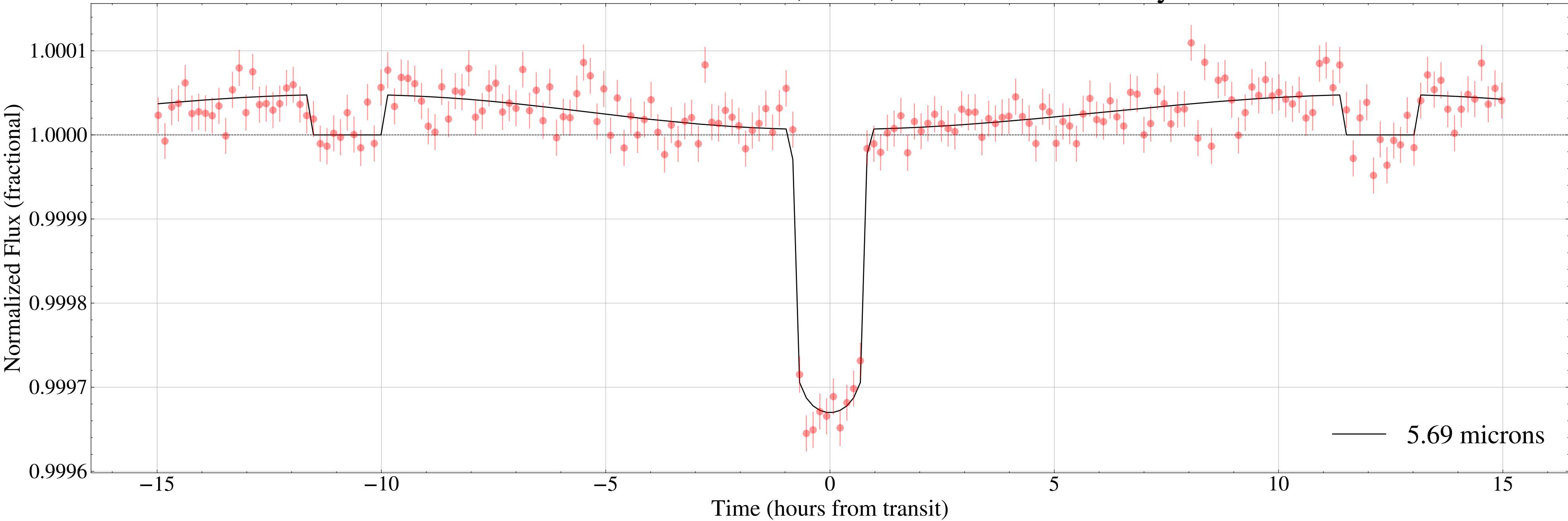
Phase curve of HD3167b; N=14, total time=13.44 days
