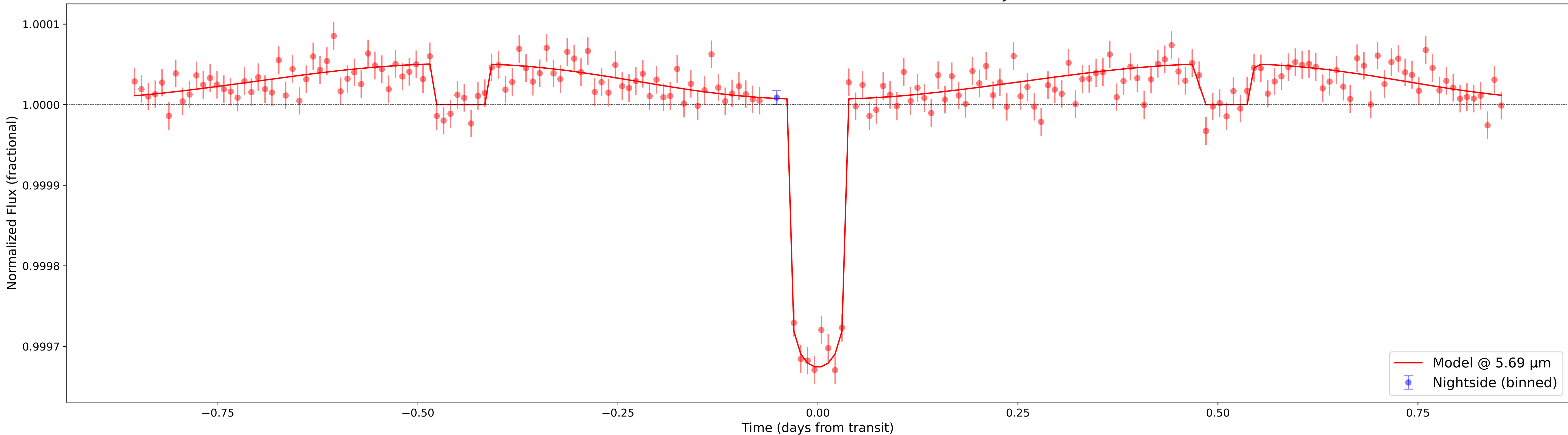
Phase curve of HD3167b; N=16, total time=15.36 days
