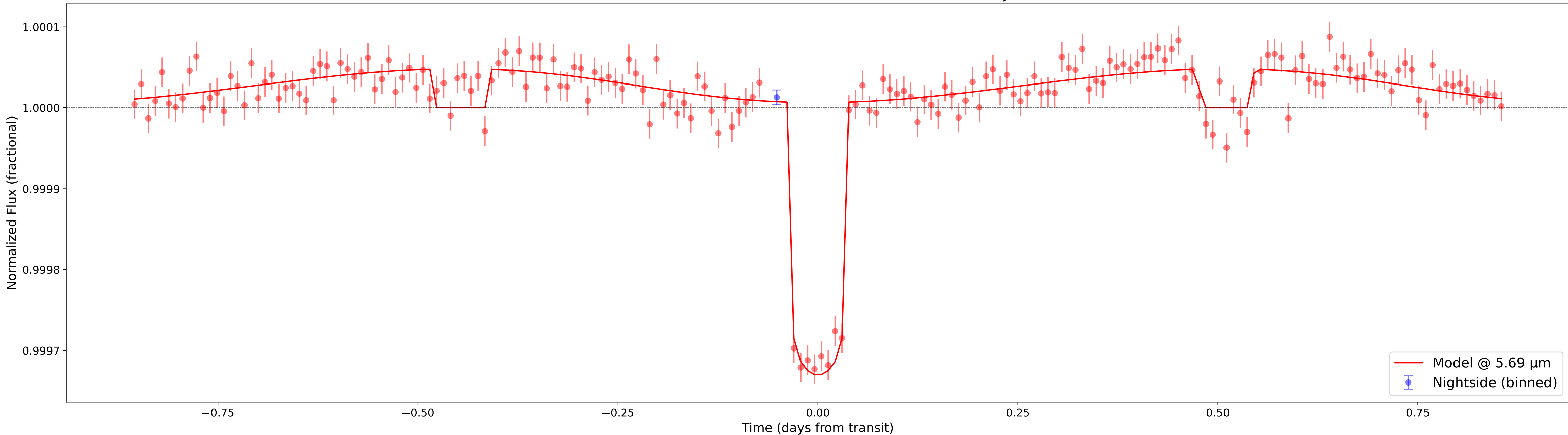
Phase curve of HD3167b; N=14, total time=13.44 days
