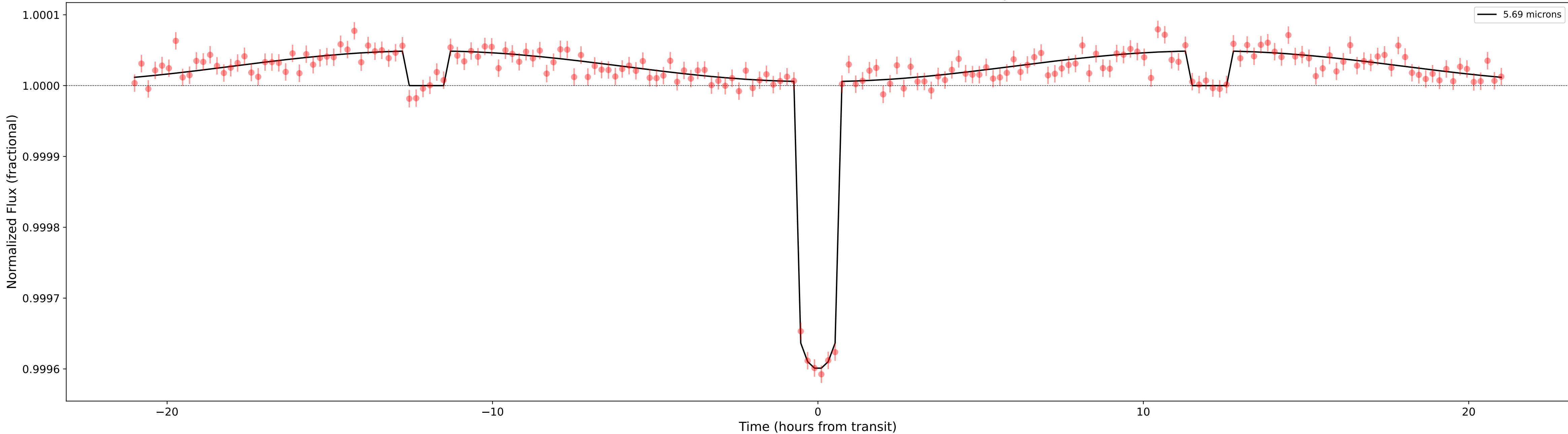
Phase curve of TOI1416b; N=51, total time=51.00 days
