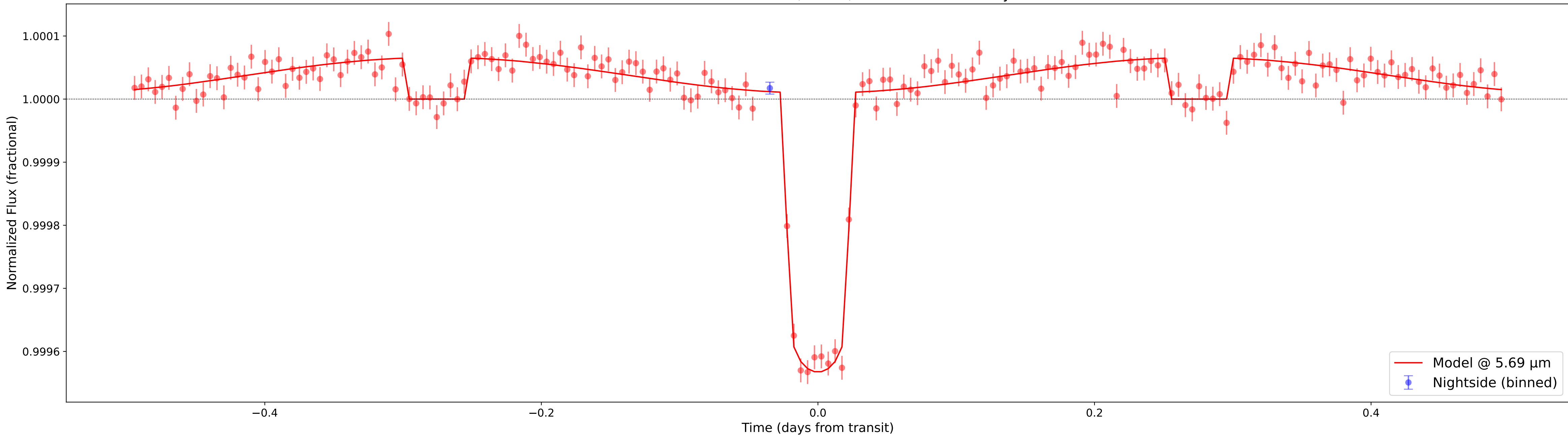
Phase curve of TOI1807b; N=26, total time=14.30 days
