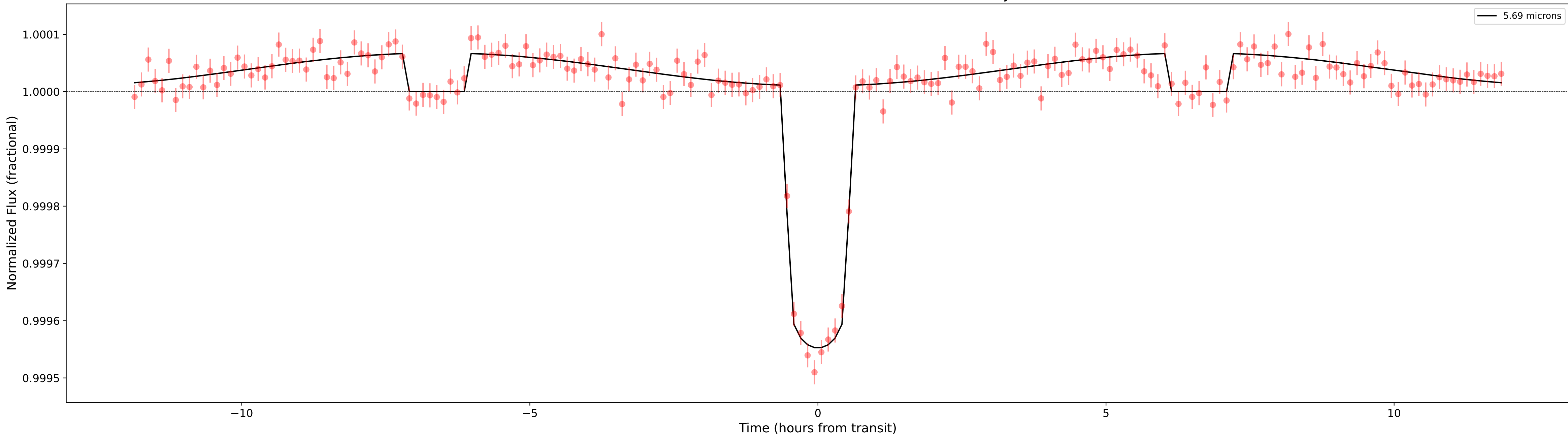
Phase curve of TOI1807b; N=21, total time=11.55 days
