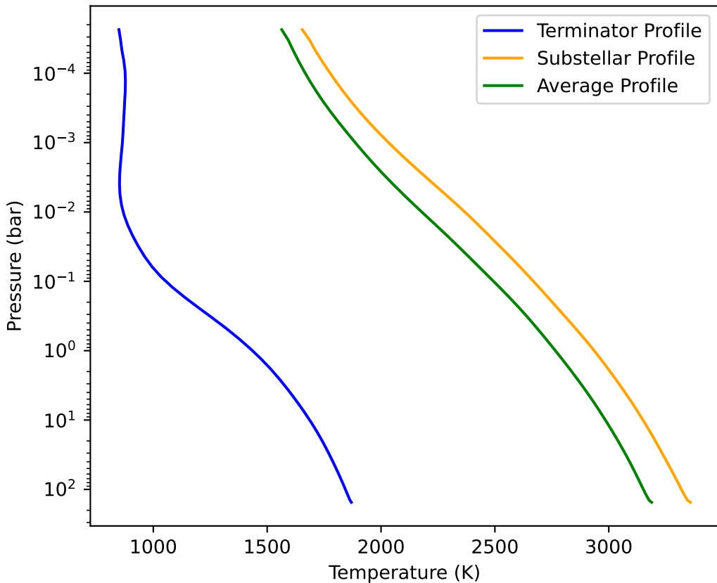
PT Profile TOI1807
