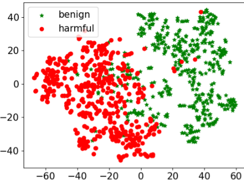
t-SNE Visualization of Noise
