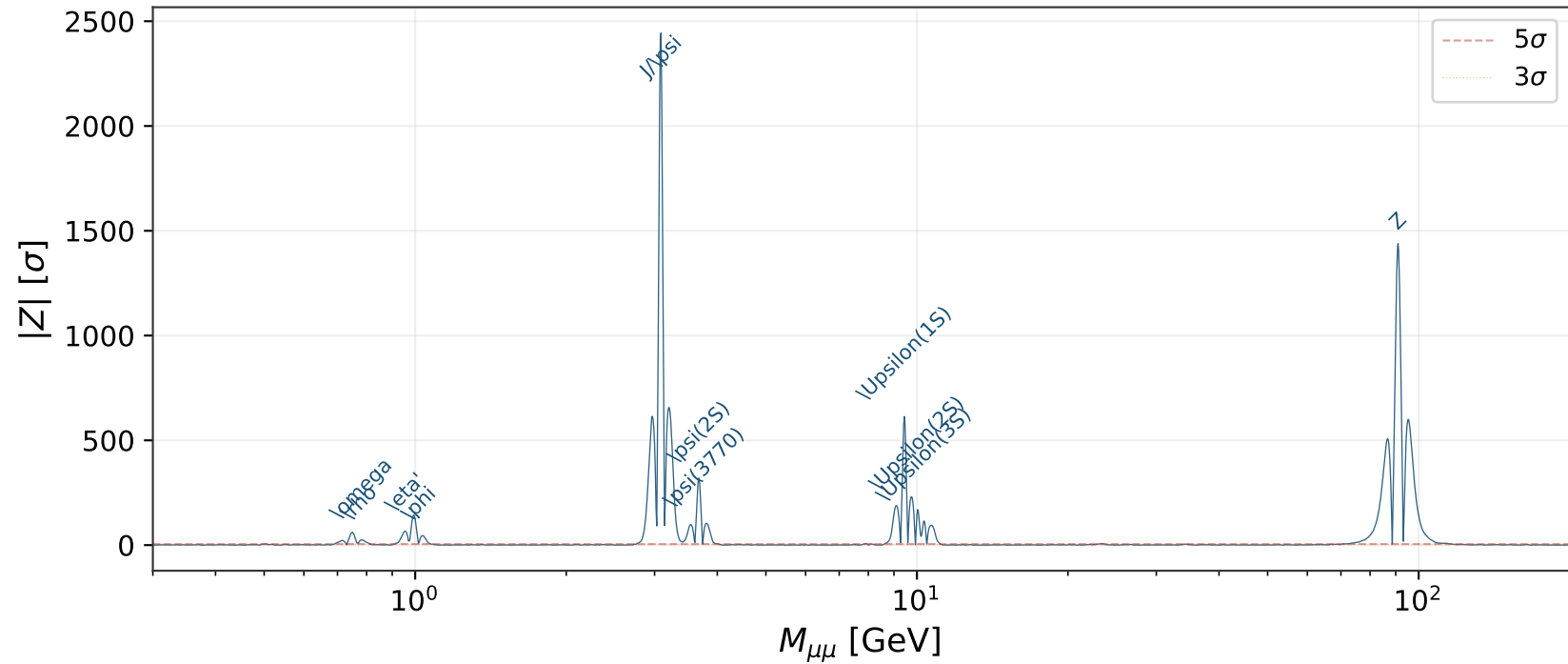
ACS Z-Score Spectrum — CMS Dimuon 13 TeV
