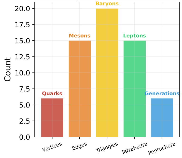
(c) 5-Simplex = Standard Model
