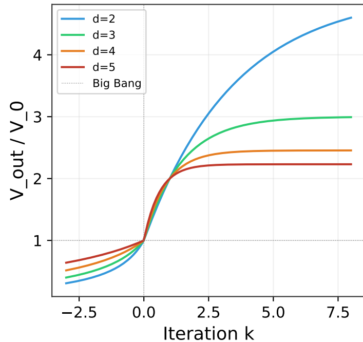
(a) Koch Volume vs k
