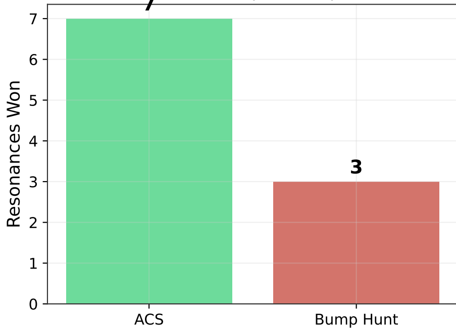
(b) ACS vs Simple Bump Hunt
