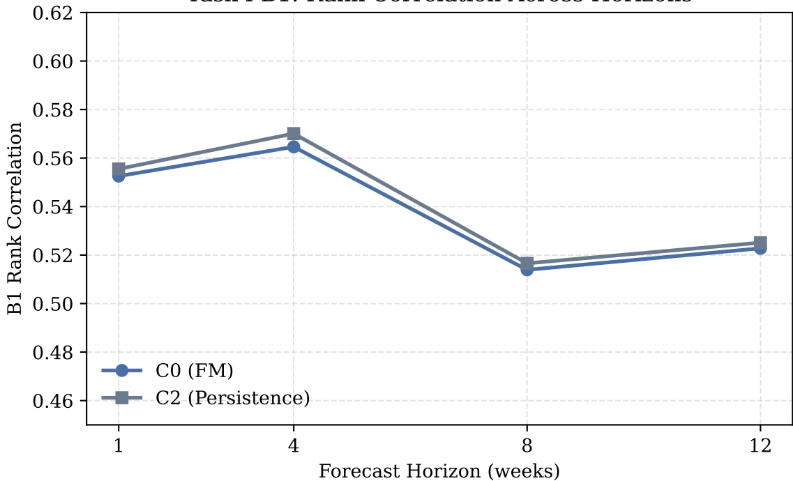
Task I B1: Rank Correlation Across Horizons
