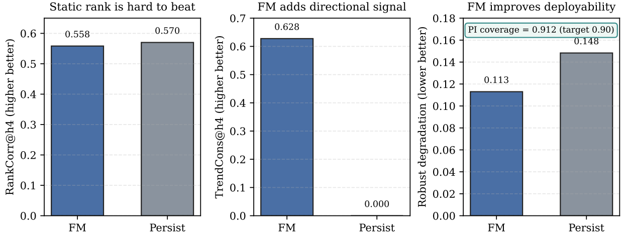
Fig. 4. Task I deployable risk signal evidence. Persistence remains a strong static-rank baseline, but the FM adds directional trend signal, maintains calibrated uncertainty, and degrades less under data corruption.
