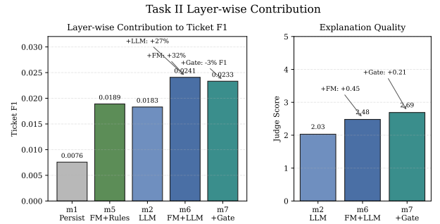
Fig. 5. Task II layer-wise contribution. Adding the FM signal to a snapshot LLM improves ticket F1 and explanation quality; replacing the FM rule engine with the LLM improves F1 further; the safety gate trades a small F1 loss for better explanations.
