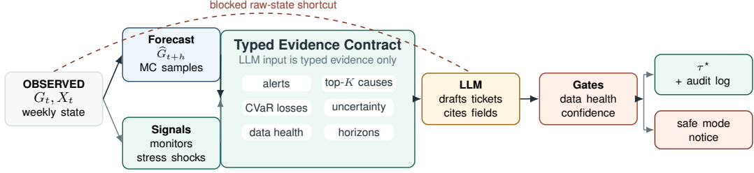
Figure 1: DeXposure-Claw system overview. A weekly exposure graph G_t is forecast into future exposure distributions and deterministic risk signals, then converted into a typed evidence contract containing monitor alerts, attribution, stress-scenario losses, uncertainty summaries, data-health signals, and forecast horizons. The LLM drafts supervisory tickets only from this structured evidence, after which data-health and confidence gates either release an auditable ticket \tau^* or enter safe mode.
