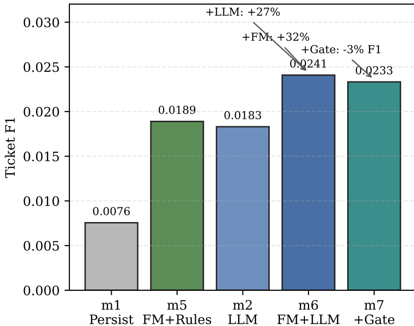
Layer-wise Contribution to Ticket F1
