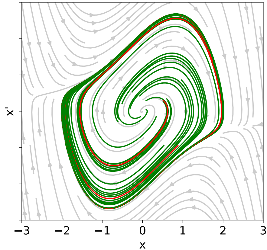
Regularized PINN
