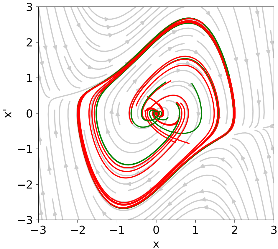
Unmodified PINN
