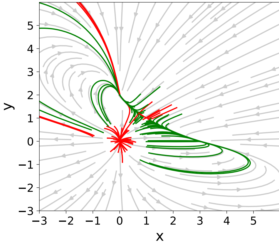
Unmodified PINN
