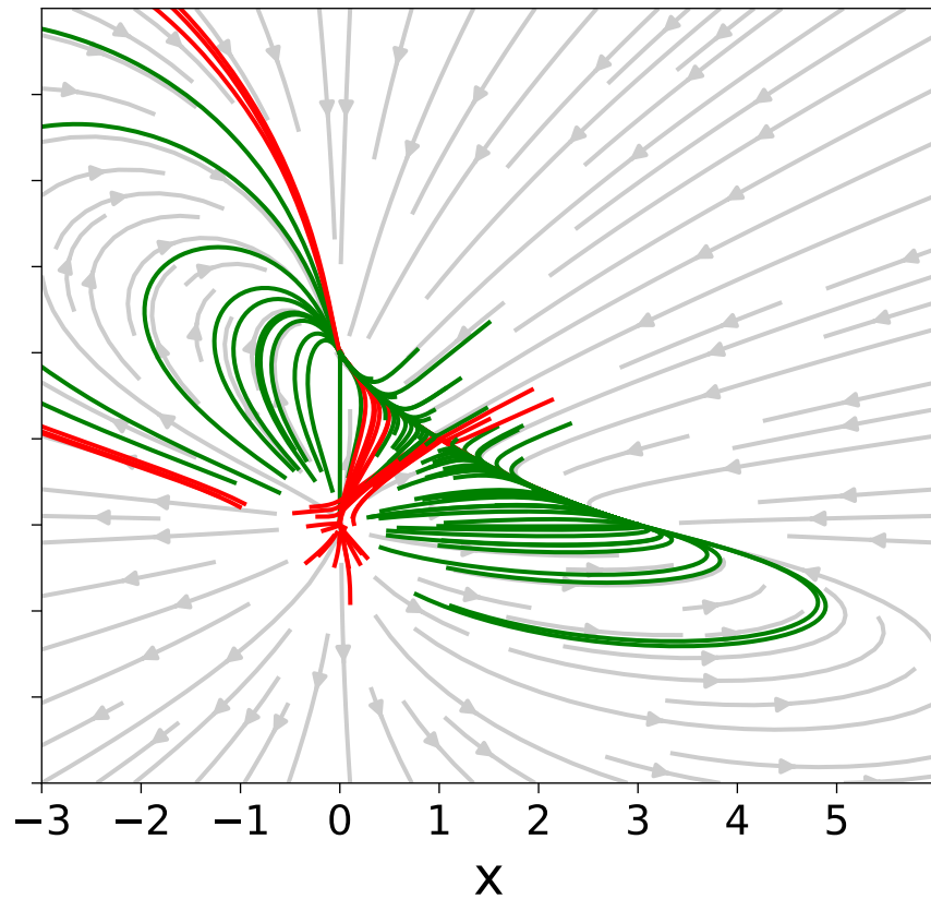
Regularized PINN
