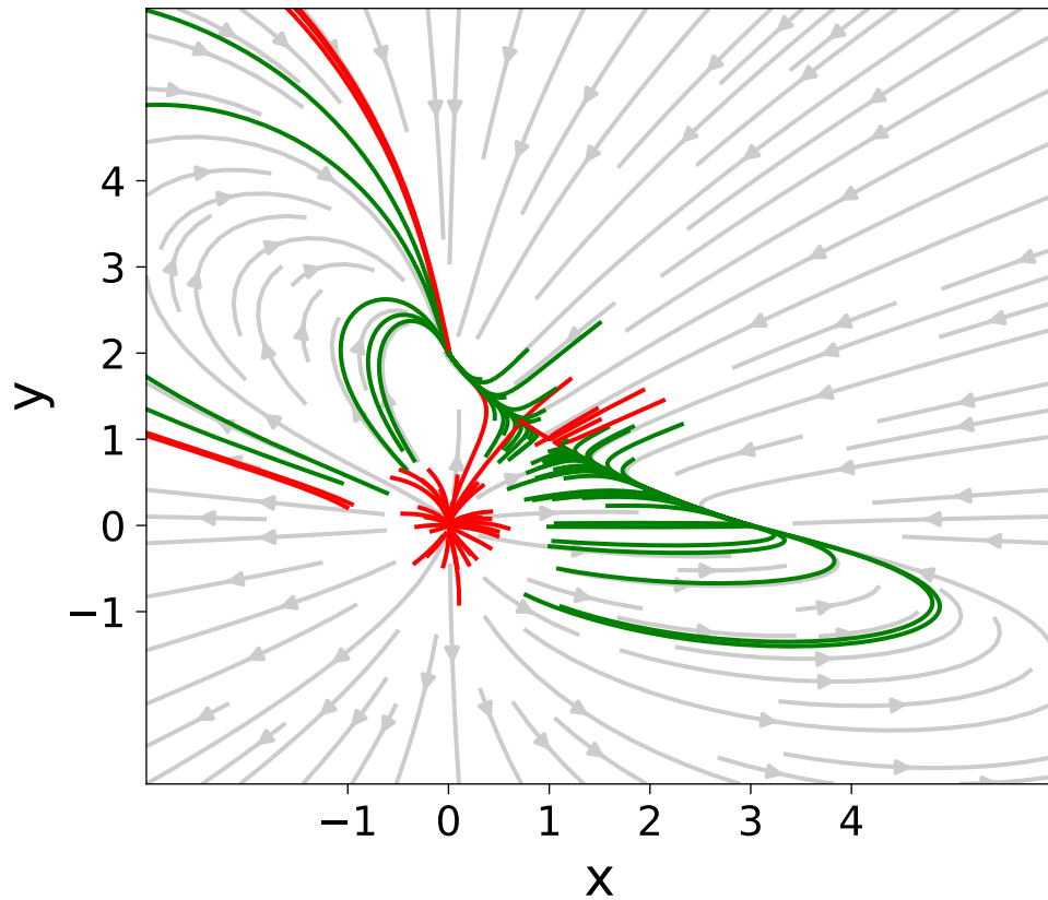
Unmodified PINN
