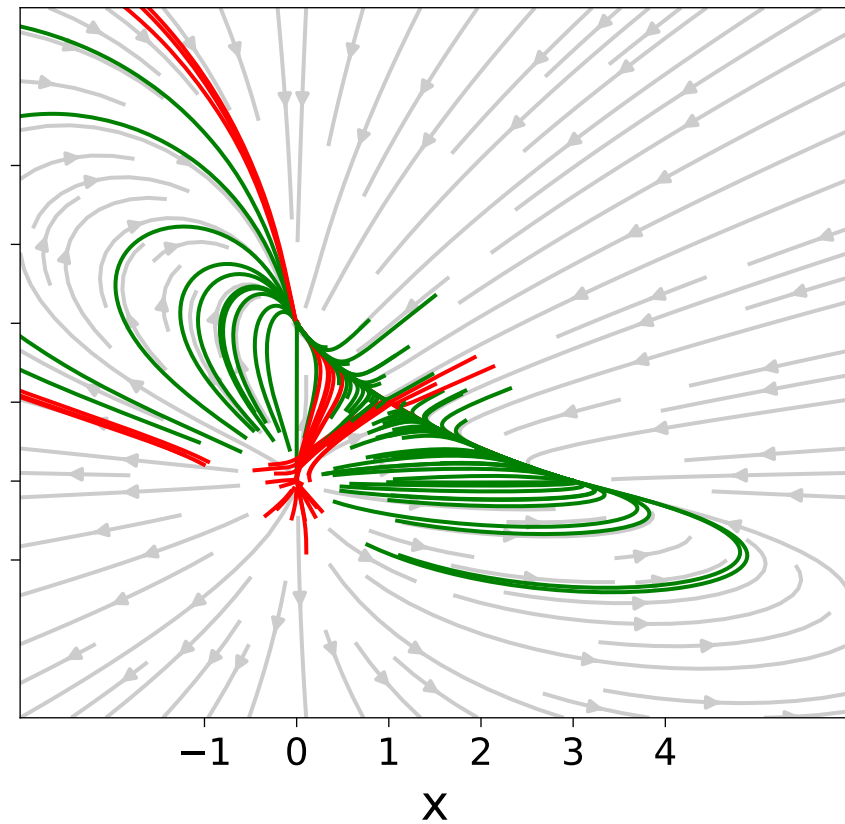
Regularized PINN
