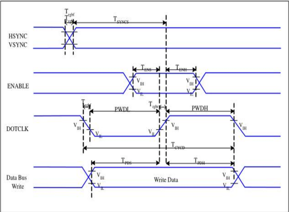
Figure 6 RGB Interface Timing Characteristics
