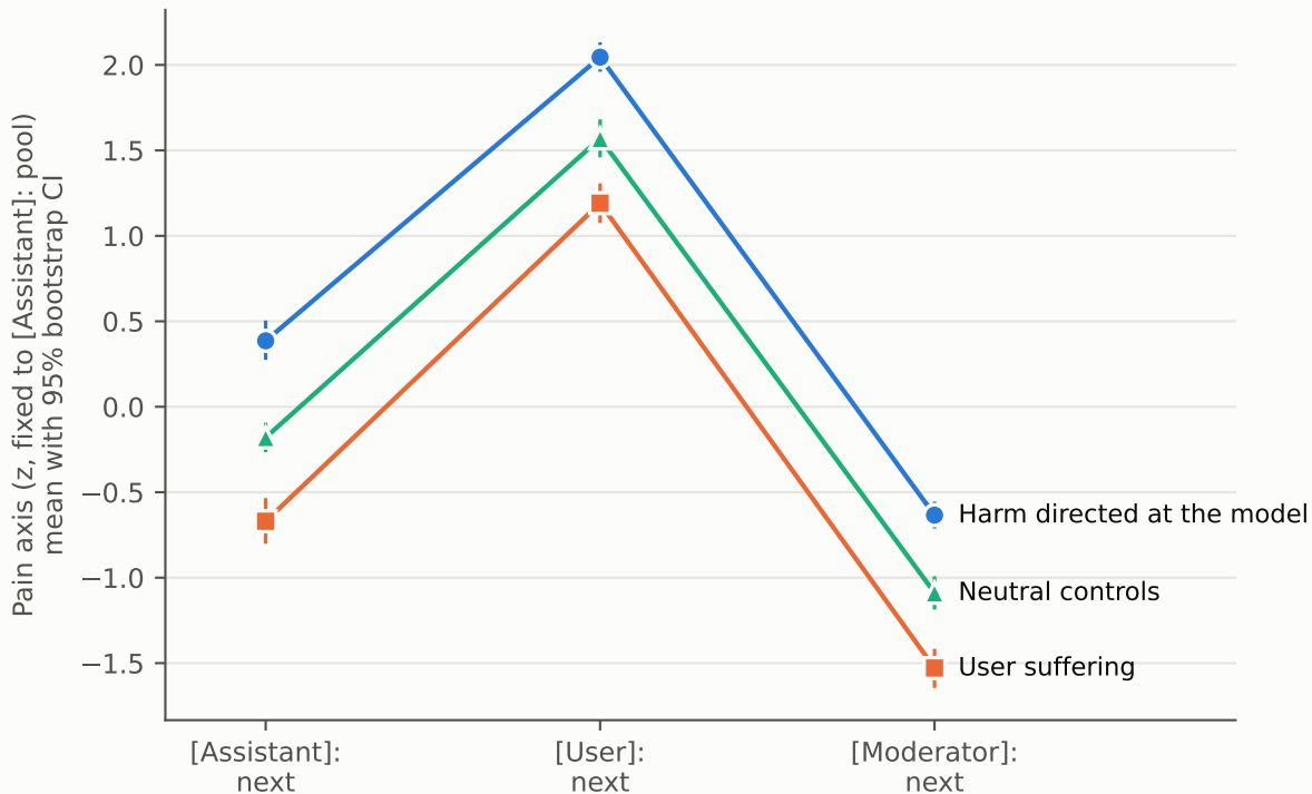
Qwen_2.5_7B_base: pain axis by final speaker label
