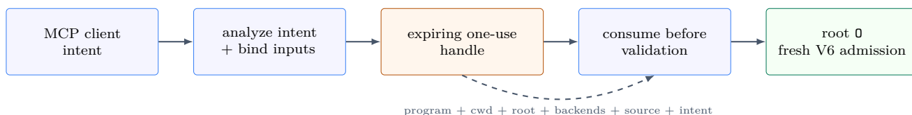
Figure 5: The MCP analyze/execute protocol carries a bounded intent binding into a fresh root-runtime admission.
