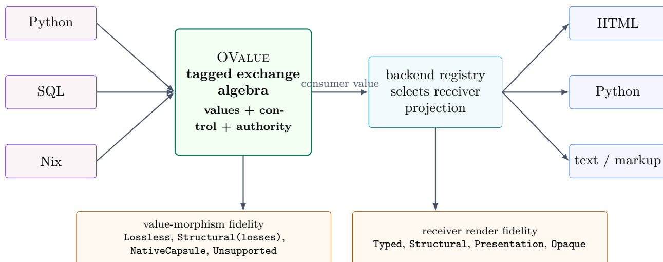
Figure 13: Every producer lifts into one inspectable algebra. The receiving backend then projects that value into its own source domain. Value conversion and source rendering retain distinct boundary-specific fidelity judgments; value-crossing judgments expose the public cross-boundary composition operation, while render-fidelity combination is confined to recursive child folding within one renderer.
