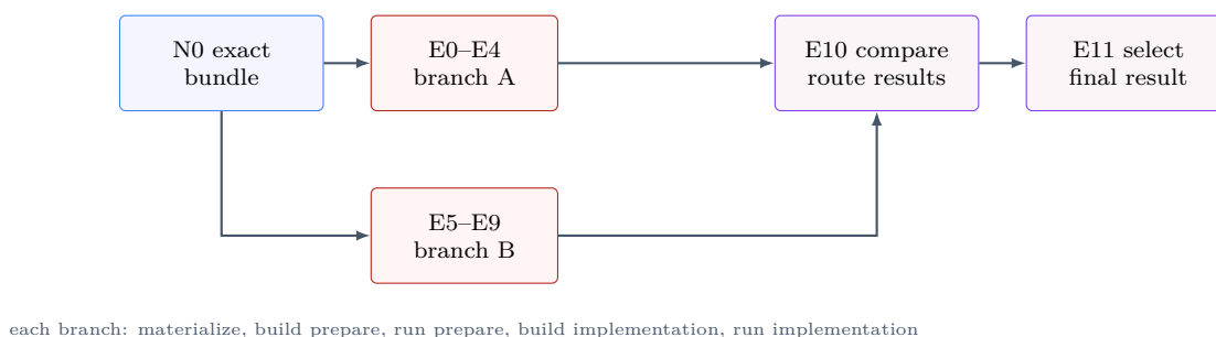
Figure 17: Reading map for the current compiler-emitted project graph. The two source-closed alternative branches converge through comparison and final selection.
