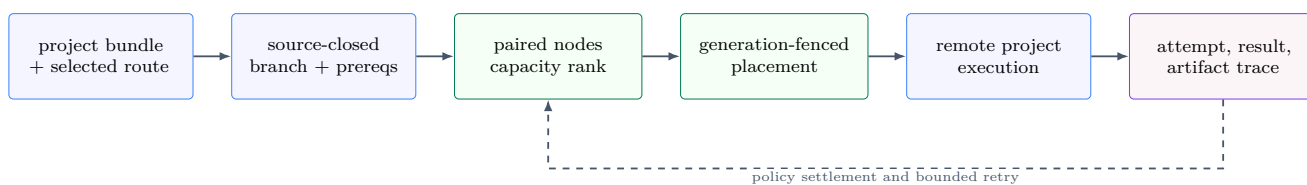
Figure 7: Project Mesh moves a complete route branch, chooses capacity, binds node generations, and returns a causally connected attempt trace.
