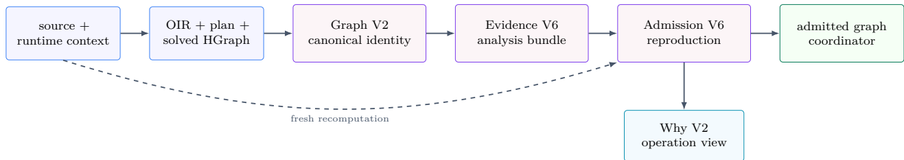
Figure 4: Current hosted execution is a proof-producing and proof-consuming pipeline. Admission reproduces the analyzer result before execution begins.
