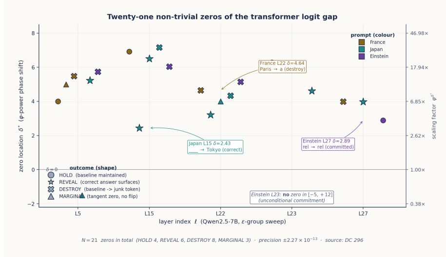
Figure 26: Twenty-one non-trivial zeros of the transformer logit gap
