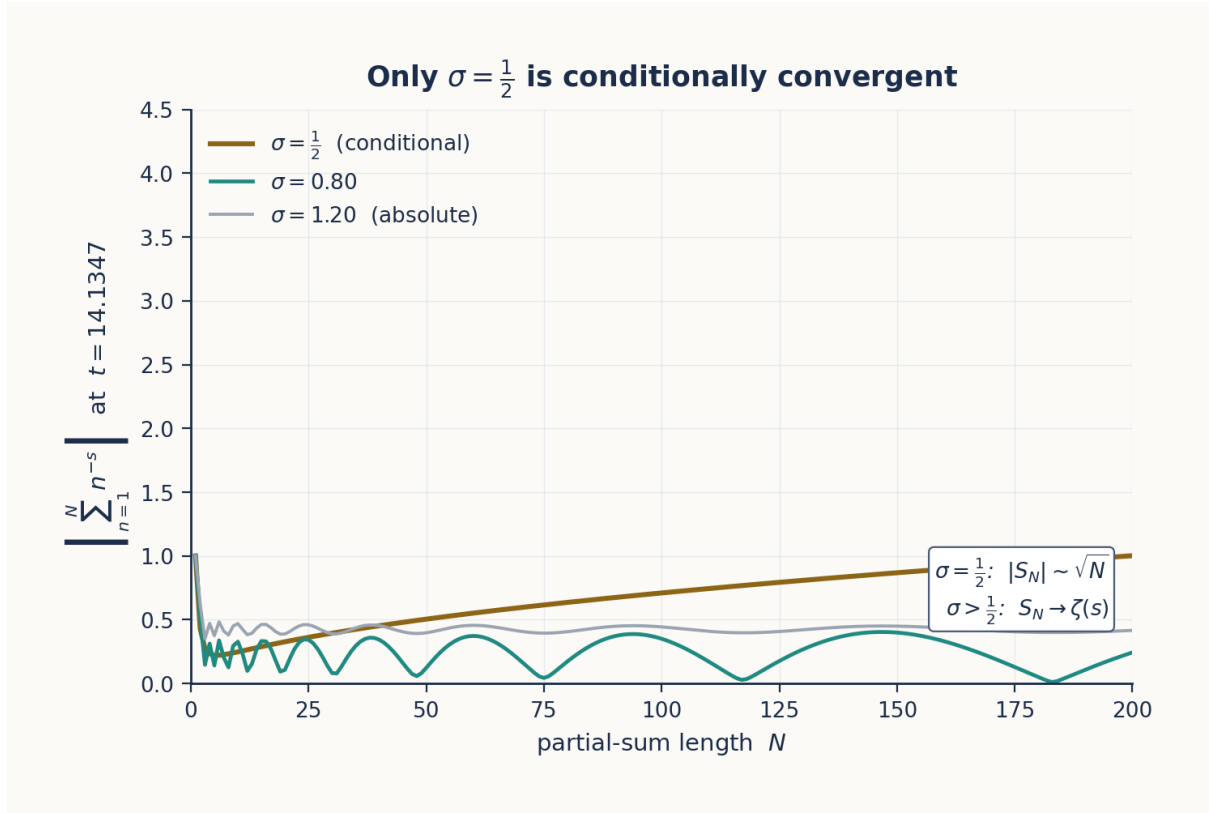
Figure B.4: Partial sums \left|\sum_{n=1}^N n^{-s}\right| at s = \sigma + 14.1347i for three amplitudes. At \sigma = 1/2 (gold) the partial sums grow as \sqrt{N} and never settle — the regime that requires Riemann-Siegel cancellation. At \sigma = 0.80 (teal) the sums oscillate but tend to a finite limit. At \sigma = 1.20 (muted) the series converges absolutely after a few terms. Only \sigma = 1/2 exhibits the conditional convergence that the Riemann-Siegel formula is built around.
