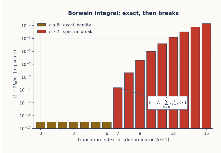
Figure 27: Borwein spectral-fragility break at n = 7
