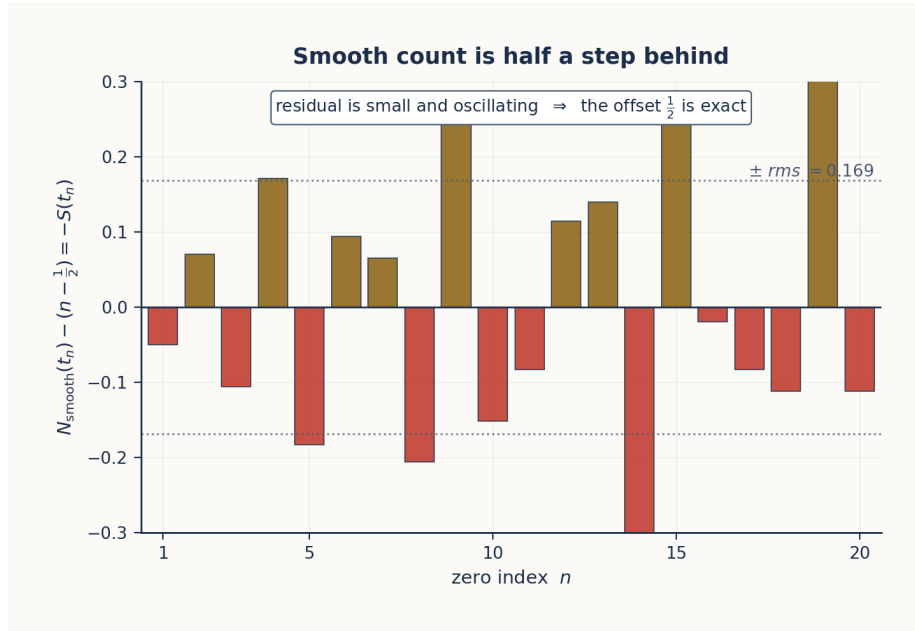
Figure 29: Half-integer offset of the smooth zero count
