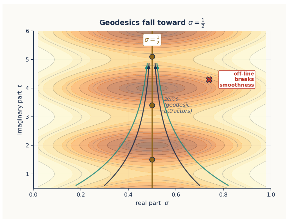
Figure 26: Geodesics on the conformal metric
