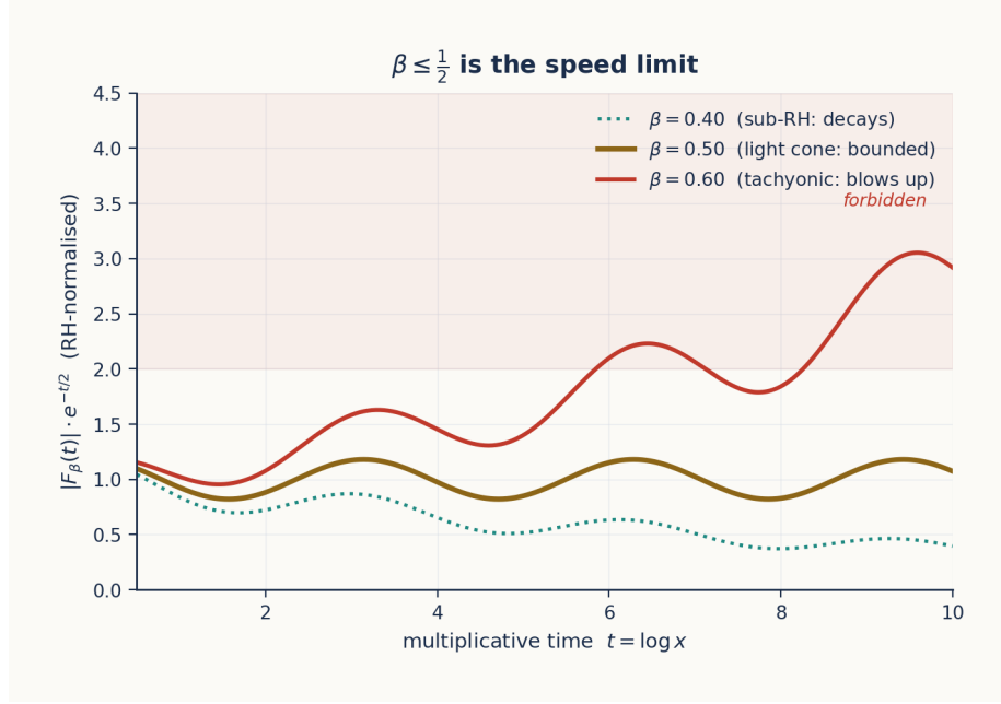
Figure 25: Light-cone constraint on the Chebyshev fluctuation
