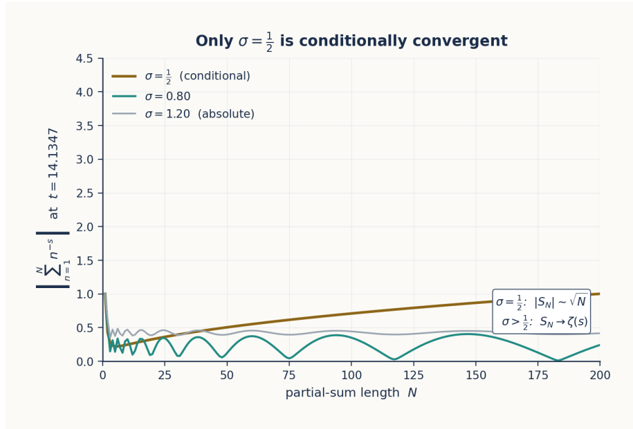
Figure 28: Conditional convergence at \sigma = 1/2
