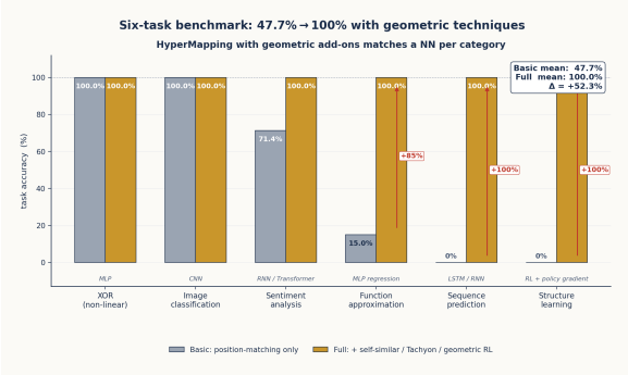
Figure 6.2: Six-task NN-capability sweep. Basic position-matching (grey) averages 47.7% across the six tasks; adding Self-Similar Transforms , Tachyon Navigation , and Geometric RL (gold) lifts every task to 100%. The three large deltas — function approximation (+85%), sequence prediction (+100%), and structure learning (+100%) — are the cases where the bare position-store fails and the geometric add-ons are what convert it into a working substitute for the conventional NN.
