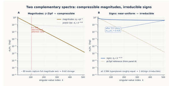
Figure 10.2: Two complementary spectral signatures of the irreducible shape. Panel A shows the MESH magnitudes’ \phi -Zipf decay \sigma_k \propto \phi^{-k} — sharp enough that \sim 89 levels suffice to capture the magnitude axis (the 8-bit storage of §7.5). The elbow at k = 106 corresponds to the discriminant-attention rank of Chapter 8 §8.3.2. Panel B shows the sign matrix’s near-uniform decay \sigma_k \propto k^{-0.14} — after 512 dimensions, \sigma_k / \sigma_1 has fallen only to 0.418. All 3,584 hyperplanes are roughly equally important, which is why the signs are irreducible* at 1 bit each.*
