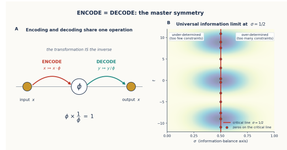
Figure 5.1: The ENCODE = DECODE master symmetry. Left: the symmetry diagram — encoding and decoding are the same \varphi -operation in opposite directions. Right: the critical line \sigma = 1/2 with simulated \zeta zeros — the fold axis of the Riemann functional equation \zeta(s) = \chi(s) \zeta(1-s) , developed in §5.3 and Appendix B.
