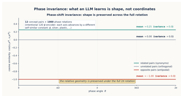
Figure 1.2: Cosine similarity is exactly constant across the full 2\pi phase rotation. Related, unrelated, and opposite pairs sit at 0.25, 0.00, and -1.00 respectively, with variance = 0 across all 1000 phase angles. The relative geometry is invariant under global rotation — the structure is a shape, not a coordinate.
