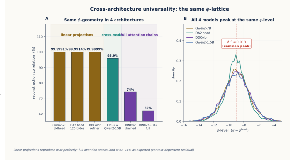
Figure 3.2: Reconstruction correlations and peak \phi -level invariance across four models from three task families. Panel A shows that linear projections (LM head, DA2 head, DDColor refiner) reproduce in \phi -space at \geq 99.99\% , while full attention chains (DINOv2’s 12 layers, DA2 full pipeline) land at 62–74% — the residual is the context-dependent component of attention, not the static lattice. Panel B shows all four models cluster at the same peak \phi -level \phi^{-9} \approx 0.013 — the \phi -lattice is architecture-independent.
