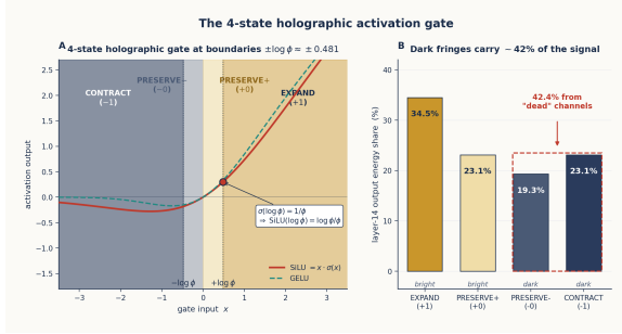
Figure 9.2: The 4-state holographic activation gate. Panel A partitions the gate input axis at boundaries \pm \log \phi \approx \pm 0.481 into four states — -1 CONTRACT, -0 PRESERVE-, +0 PRESERVE+, +1 EXPAND — and shows SiLU and GELU passing through the field. The identity \sigma(\log \phi) = 1/\phi pins the boundaries to \phi exactly. Panel B shows the energy contribution by state at Qwen2-7B layer 14: the two “dead” PRESERVE channels together account for 42.4% of the output energy. Removing the -0 state collapses end-to-end argmax from 4/5 to 0/5 on the verification suite — the dark fringes are not a stylistic distinction, they carry the holographic-image content.
