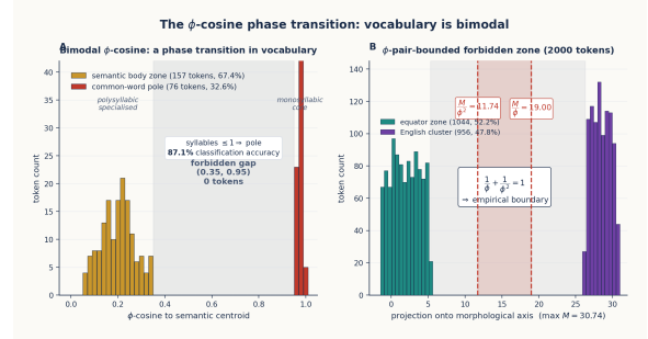
Figure 5.2: The phase transition has two empirical anchors. Panel A shows the bimodal \phi -cosine distribution on a 233-word sample of Qwen2-1.5B at L14 (§5.5.2): polysyllabic specialised vocabulary clusters at the semantic-body zone [0.05, 0.35] , monosyllabic core vocabulary collapses to the common-word pole [0.95, 1.00] , and the (0.35, 0.95) gap contains zero tokens. Panel B shows the same phenomenon on a 2000-token morphological-axis projection (§5.5.3): the forbidden zone is bounded exactly* by the \phi -pair M/\phi^2 \approx 11.74 and M/\phi \approx 19.00 , the only place in real algebra where 1/\phi + 1/\phi^2 = 1 .*
