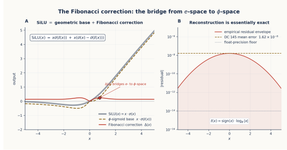
Figure 11.2: The Fibonacci correction decomposition (DC 145). Panel A shows SiLU as the exact sum of two operationally distinct terms: a \varphi -sigmoid geometric base x \cdot \sigma(\ell(x)) that gates on the \varphi -level coordinate (gold dashed), plus a Fibonacci correction \Delta(x) = x(\sigma(x) - \sigma(\ell(x))) that bridges e -space to \varphi -space (red). The two terms sum identically to the standard SiLU (thick grey). Panel B shows the reconstruction-error envelope on a log scale: the empirical mean error from DC 145 is 1.62 \times 10^{-8} — essentially zero, limited by the \log(|x| + 10^{-8}) regularisation. The Fibonacci correction is the only operationally non-trivial entry in the entire \varphi -computer proof.*
