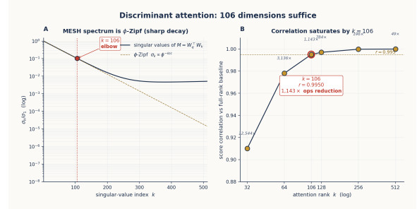
Figure 8.2: Discriminant attention rank k = 106 derived from the MESH spectrum. Panel A shows the MESH singular values follow a \phi -Zipf decay \sigma_k \propto \phi^{-k} — sharp enough that the top \sim 100 singular vectors capture nearly all the variance. Panel B shows the corresponding score correlation against the full-rank baseline as k varies on the verification sweep \{32, 64, 106, 128, 256, 512\} : the elbow is at k = 106 with r = 0.9950 and a 1,143\times ops reduction.
