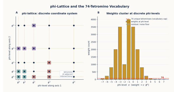
Figure 7.1: Left: The \phi -lattice — a 2D projection showing grid lines at \phi -power intervals. Each intersection is a valid weight coordinate. Right: Weight count by \phi -level, showing clustering at discrete levels with 74 unique tetromino structures.
