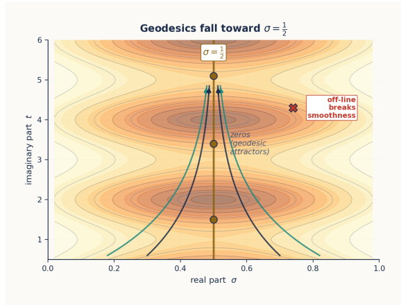
Figure B.2: Geodesics on the conformal metric e^{2\Phi(s)} where \Phi(s) = \frac{1}{2} \log |\zeta(s)\zeta(1-s)| . The metric level sets (orange contours) form a parabolic well centred on \sigma = 1/2 ; geodesics from starting points off the line fall toward it as if into an attractor basin. Critical-line zeros (gold dots) are smooth termination points; an off-line zero (red X) immediately breaks completeness.
