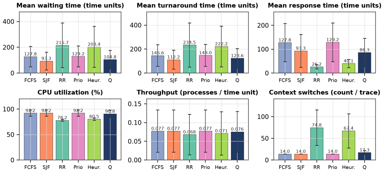
Figure 7.1: Six metrics on the held-out test set (error bars = SD across workloads).
