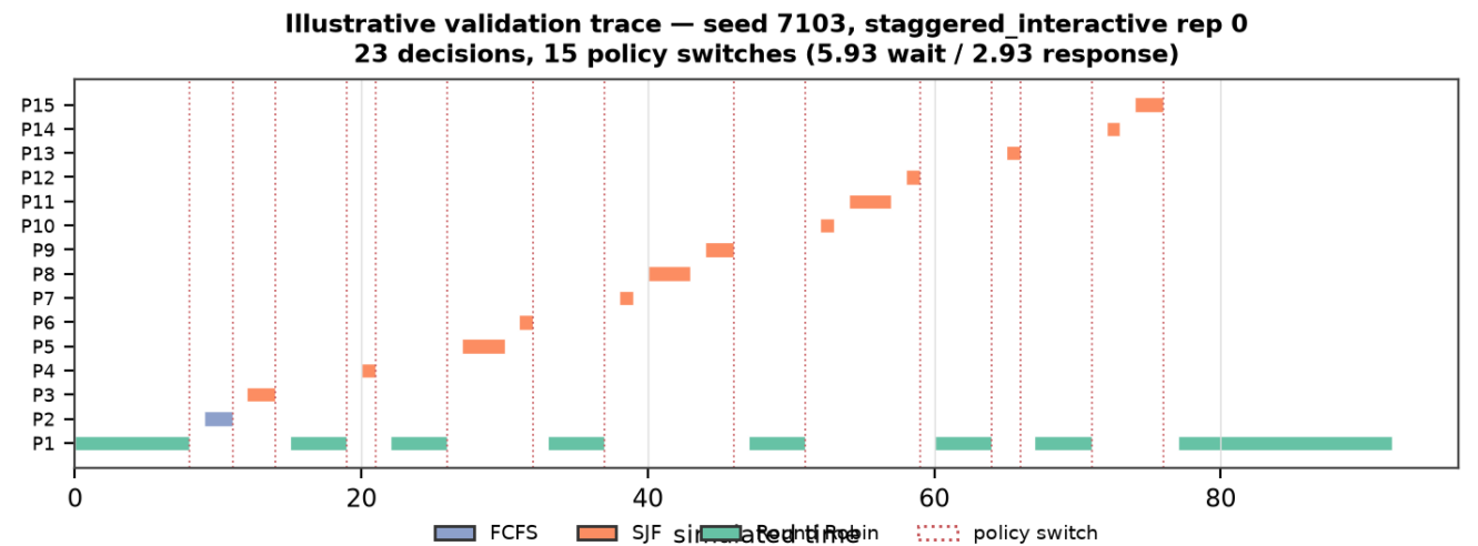
Figure 8.2: Illustrative trace. Bars are execution segments coloured by the policy chosen for them; dotted lines mark the instants where the policy changed.
