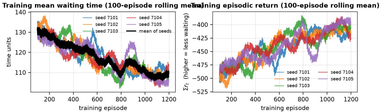
Figure 7.2: Sequential training: rolling mean waiting time and episodic return (100-episode window) for each of the five agents.
