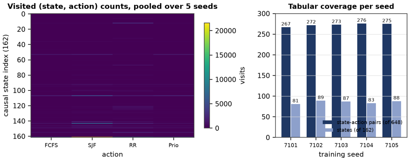
Figure 8.1: Learned state-action visitation pooled over the five agents (left) and per-seed coverage (right). Between 267 and 276 of the 648 pairs are visited.
