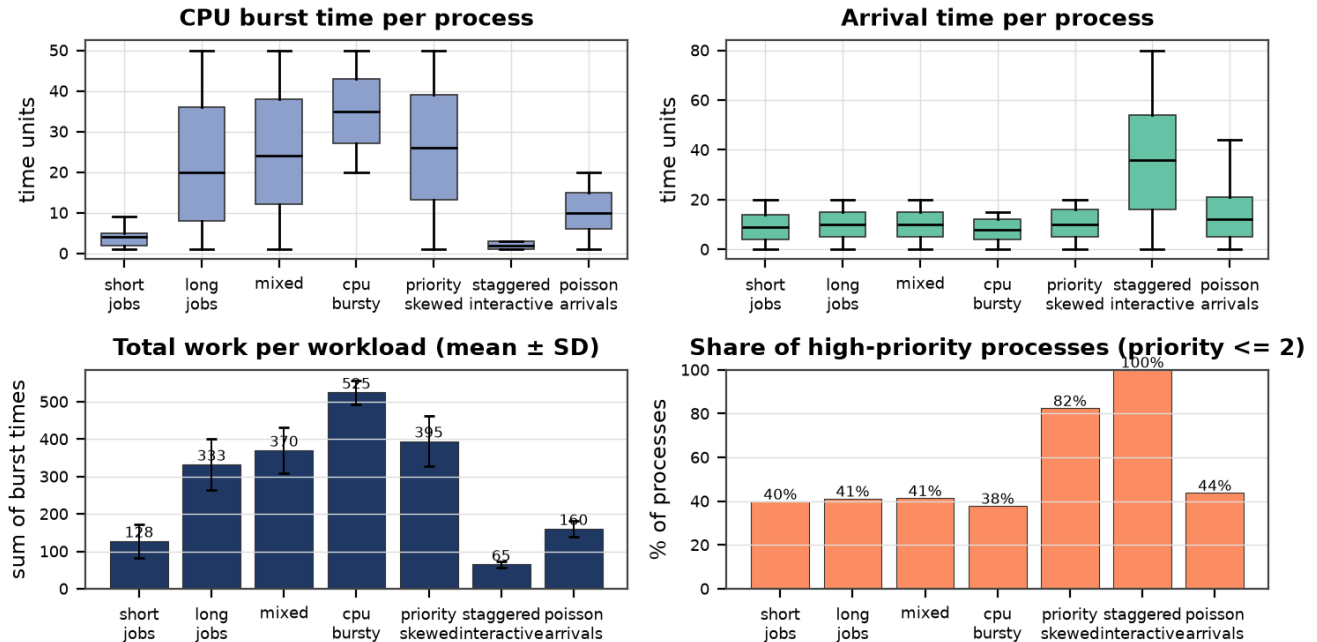
Figure 5.1: Profile of the generated held-out dataset: burst-time and arrival-time spread per family, total work per workload and high-priority share.
