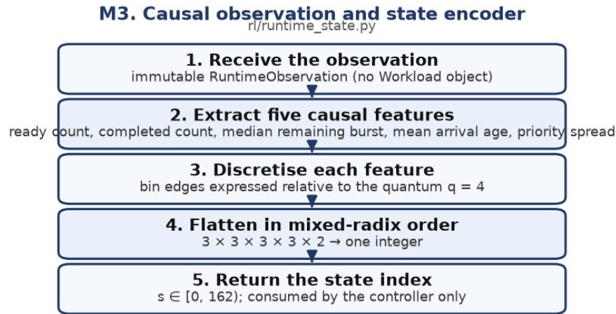
Figure 4.3: Workflow of Causal observation and state encoder.
