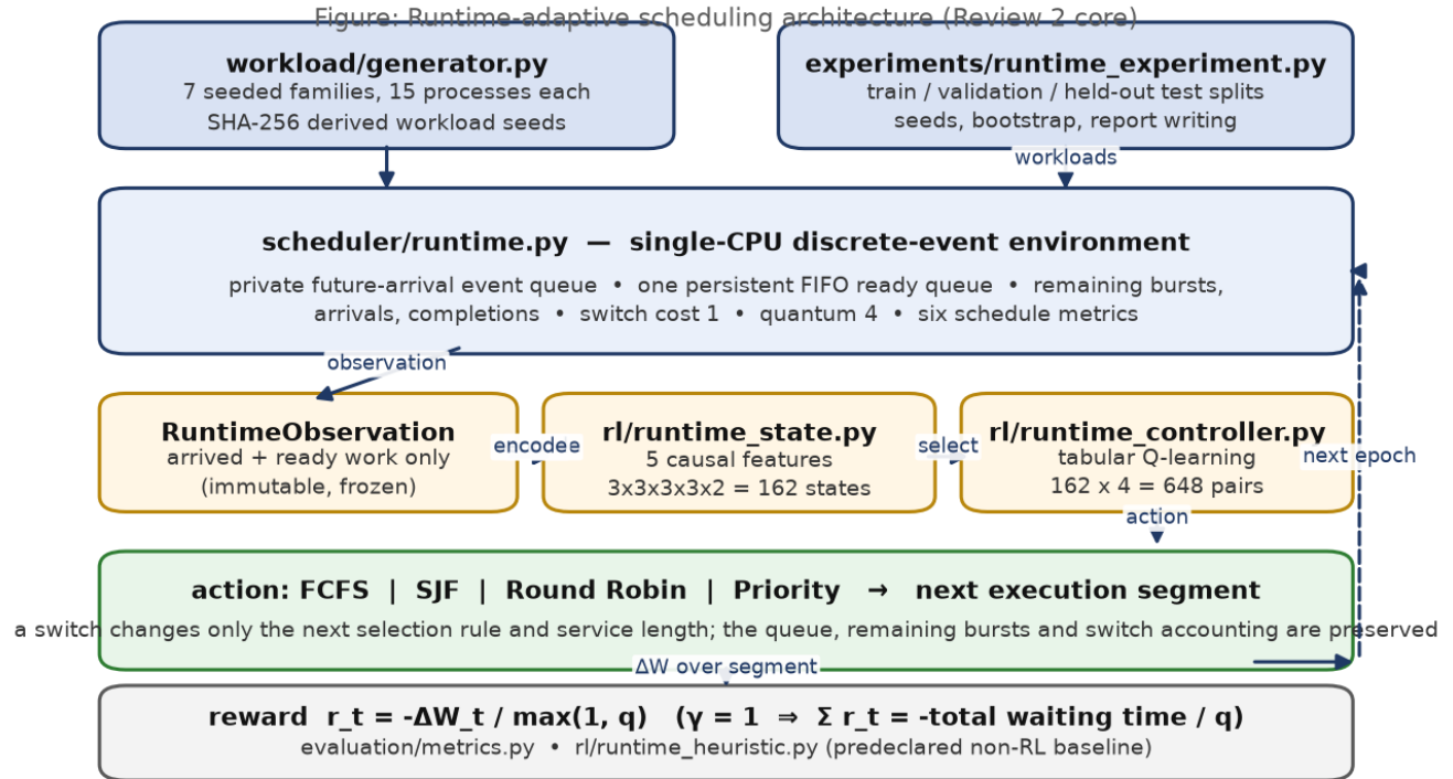
Figure 2.1: Conceptual architecture. Blue = environment (owns future arrivals, ready queue and switch accounting); amber = controller path (arrived work only); green = the action returned to the environment.
