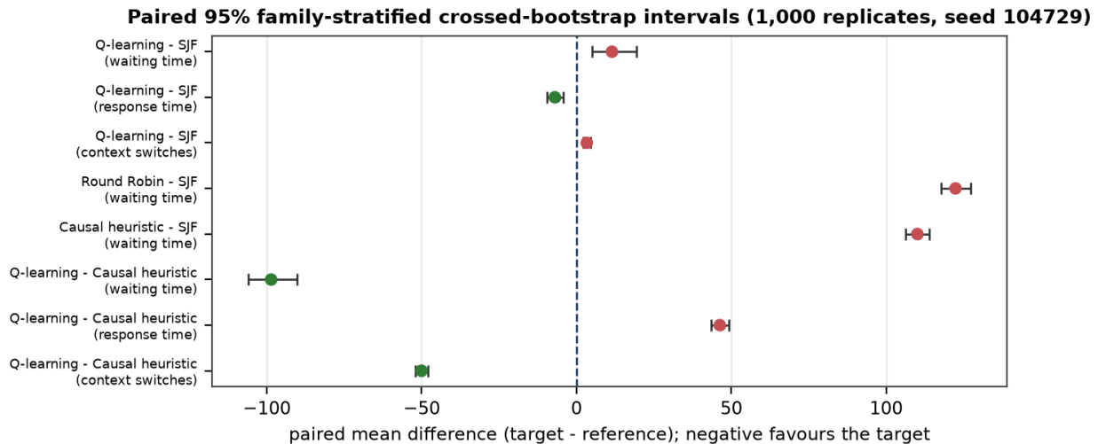
Figure 7.3: Forest plot of the paired comparisons (green favours the target, red favours the reference).
