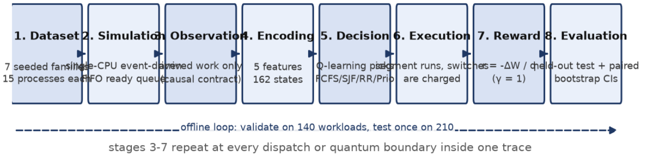
Figure 1.1: Methodology pipeline. Stages 3–7 form the online decision loop; stage 8 is the offline evaluation that produces every number reported here.
