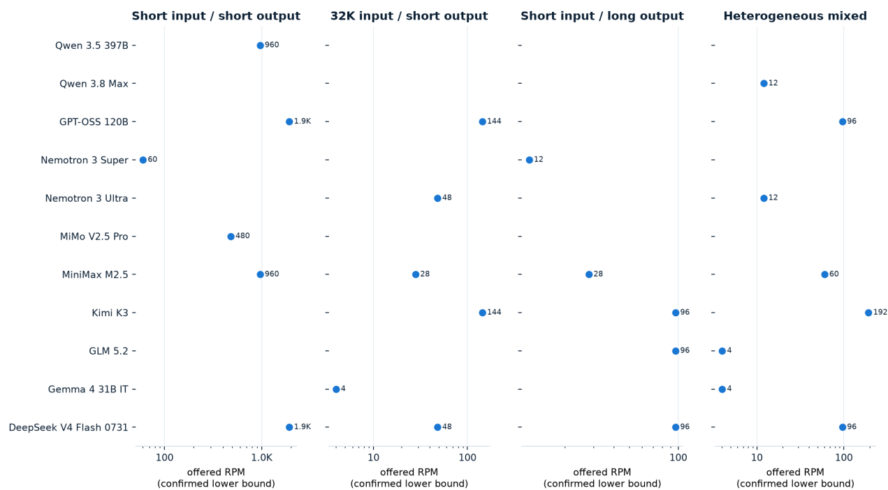
AIMD healthy offered-rate lower bounds — matched workload cells
