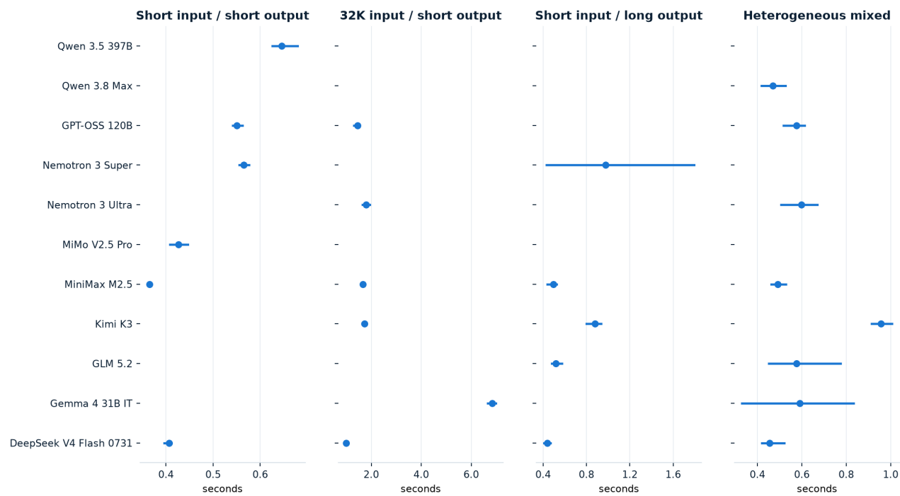
Median time to first streamed token at the confirmed AIMD cell
