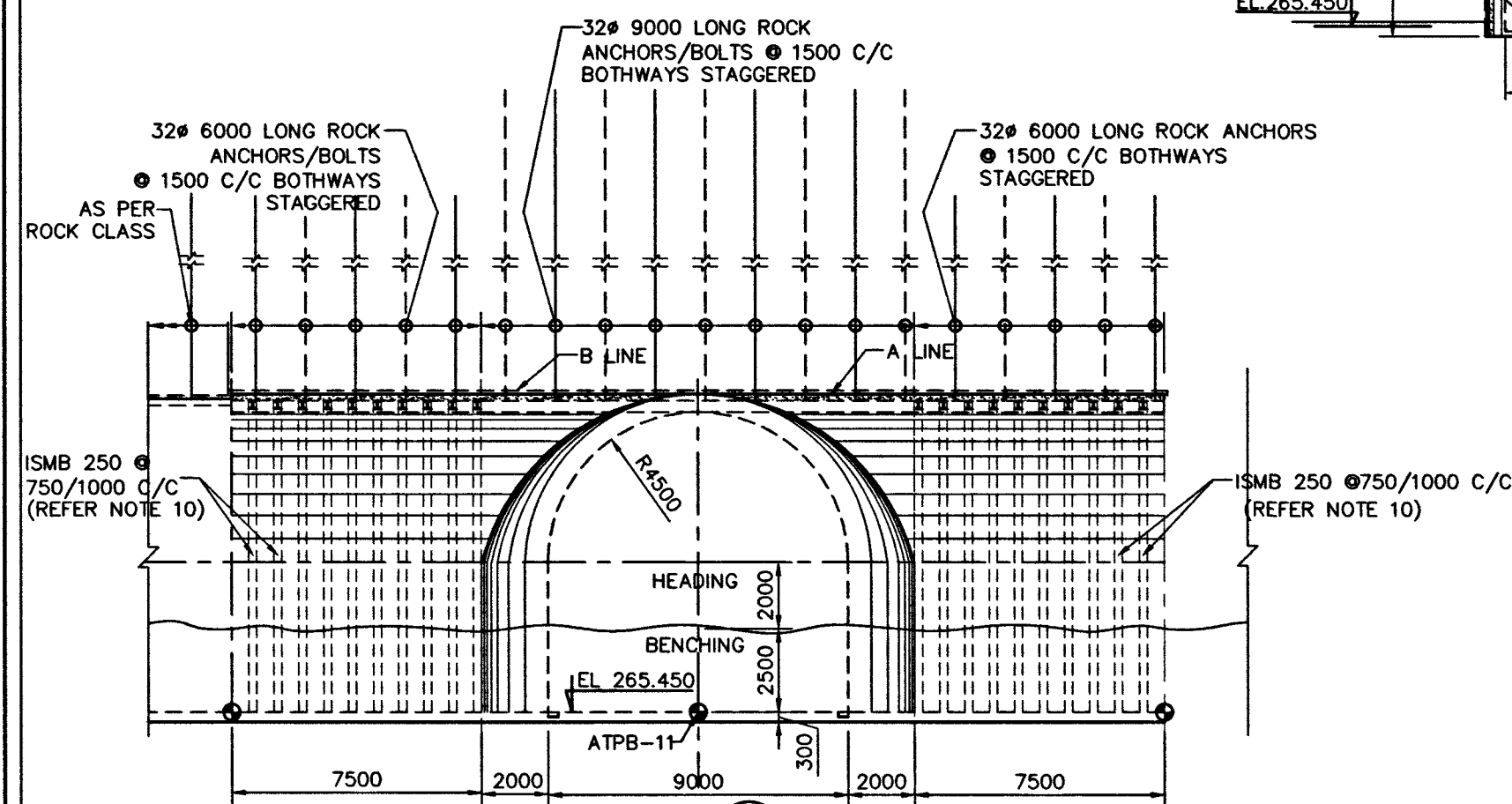
SECTION A
