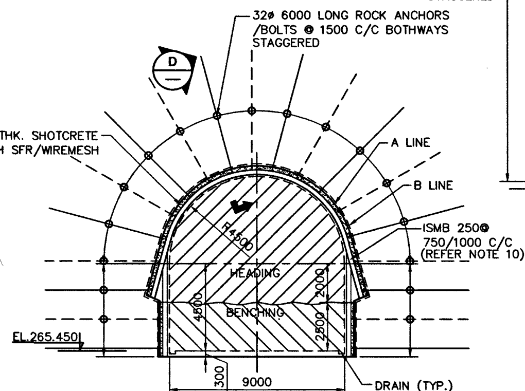
SECTION C
