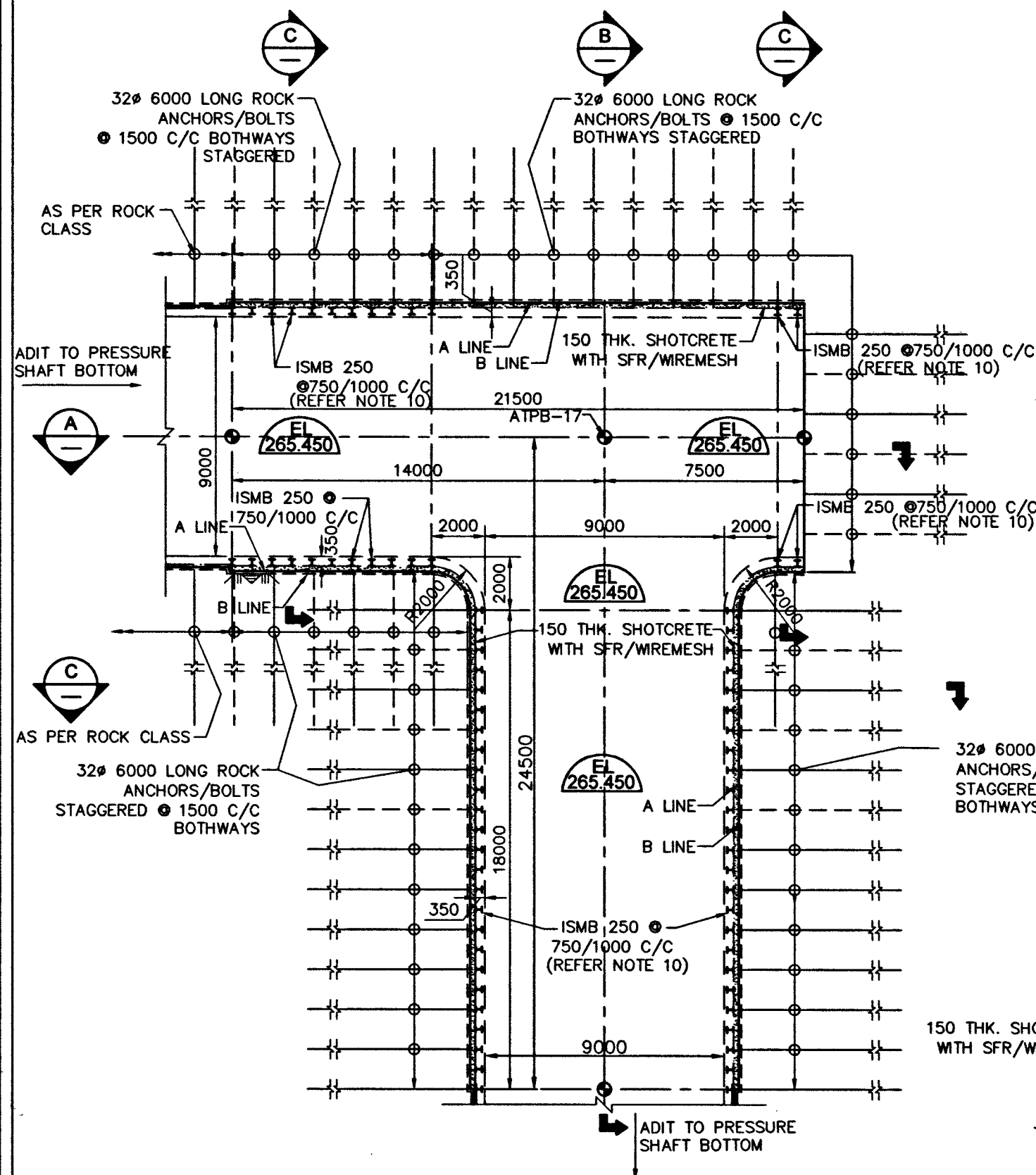
TYPICAL PLAN FOR ADIT TO PRESSURE SHAFT BOTTOM JUNCTION 6
