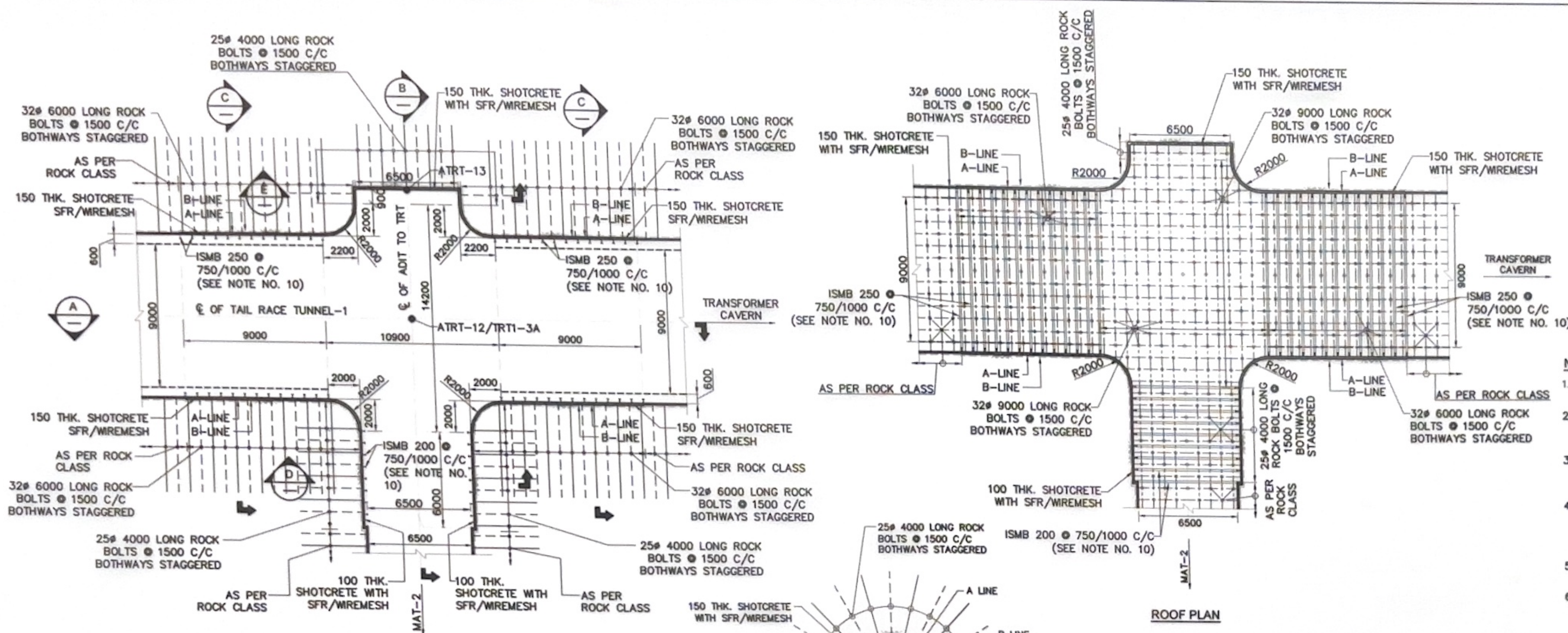
TYPICAL PLAN OF JUNCTION FOR TAIL RACE TUNNEL - 1
