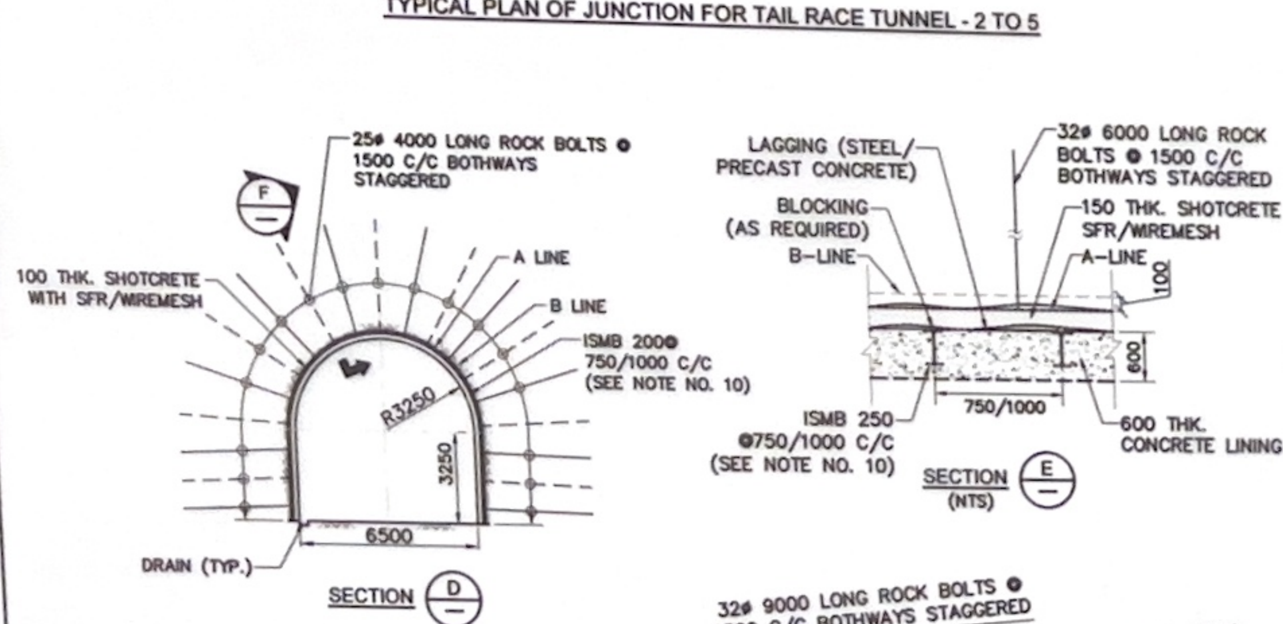
TYPICAL PLAN OF JUNCTION FOR TAIL RACE TUNNEL - 2 TO 5
