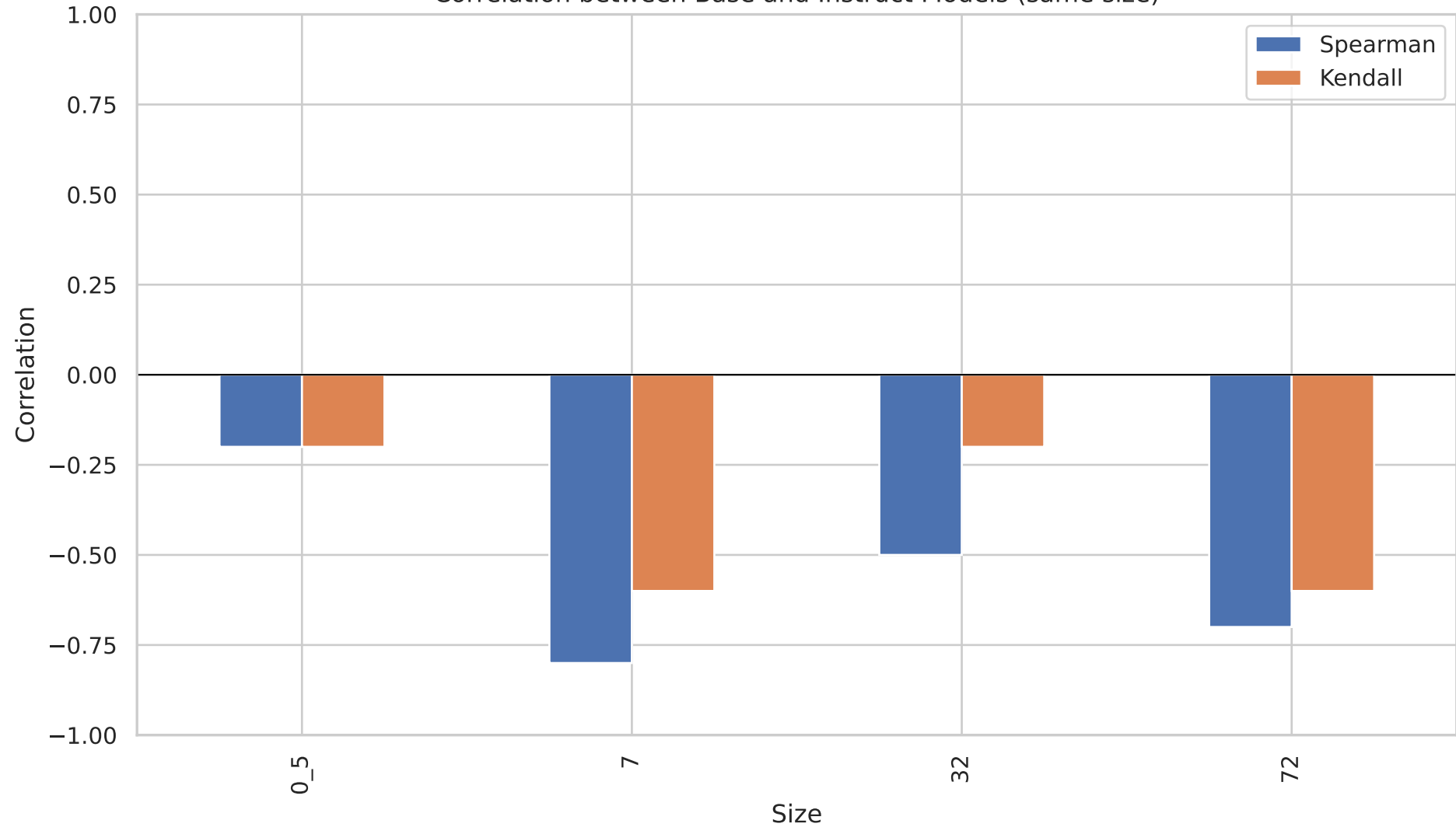
Correlation between Base and Instruct Models (same size)
