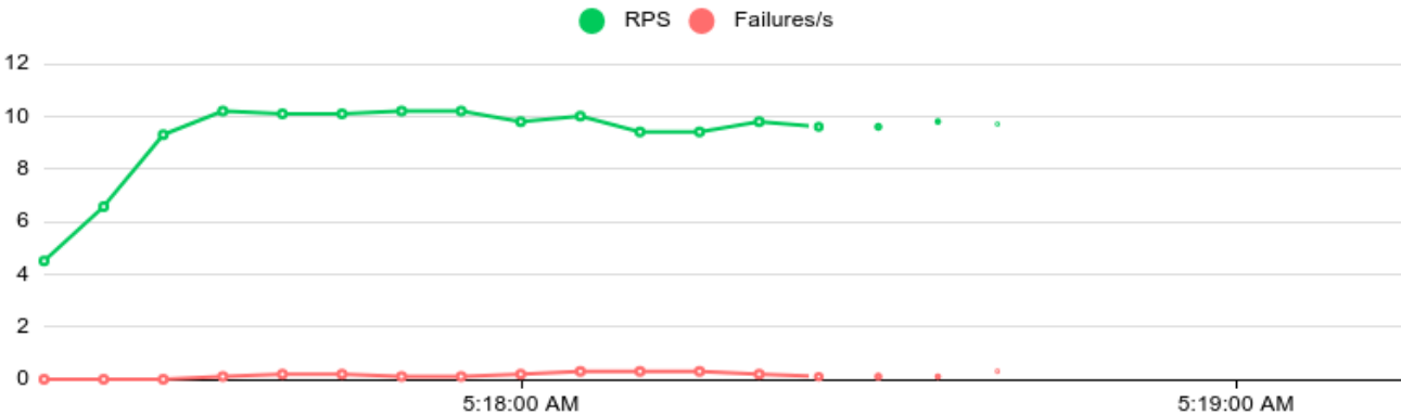
Total Requests per Second
