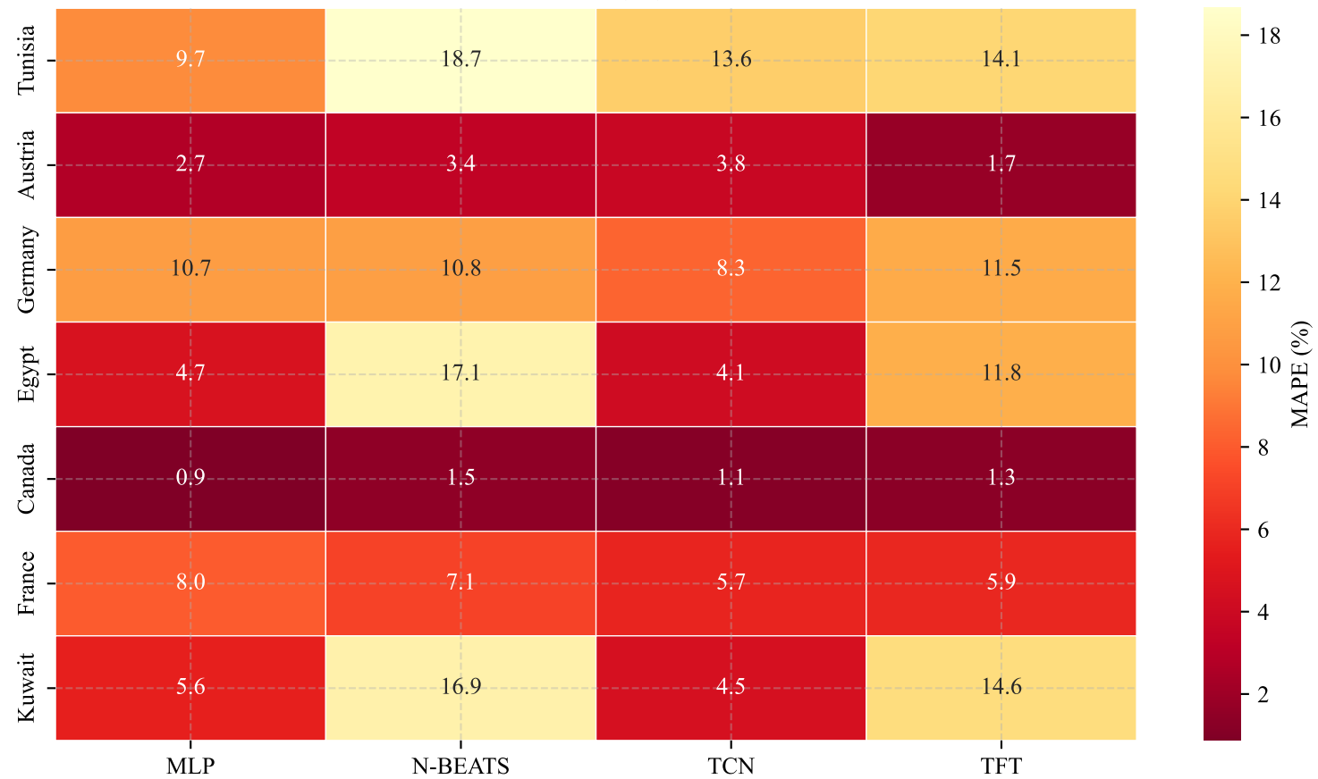
DL Model MAPE (%) — Test Set
