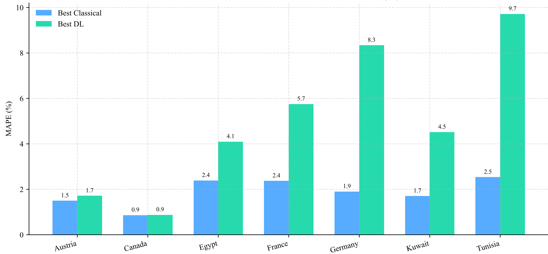
Best Classical vs Best DL Model — Test MAPE (%)
