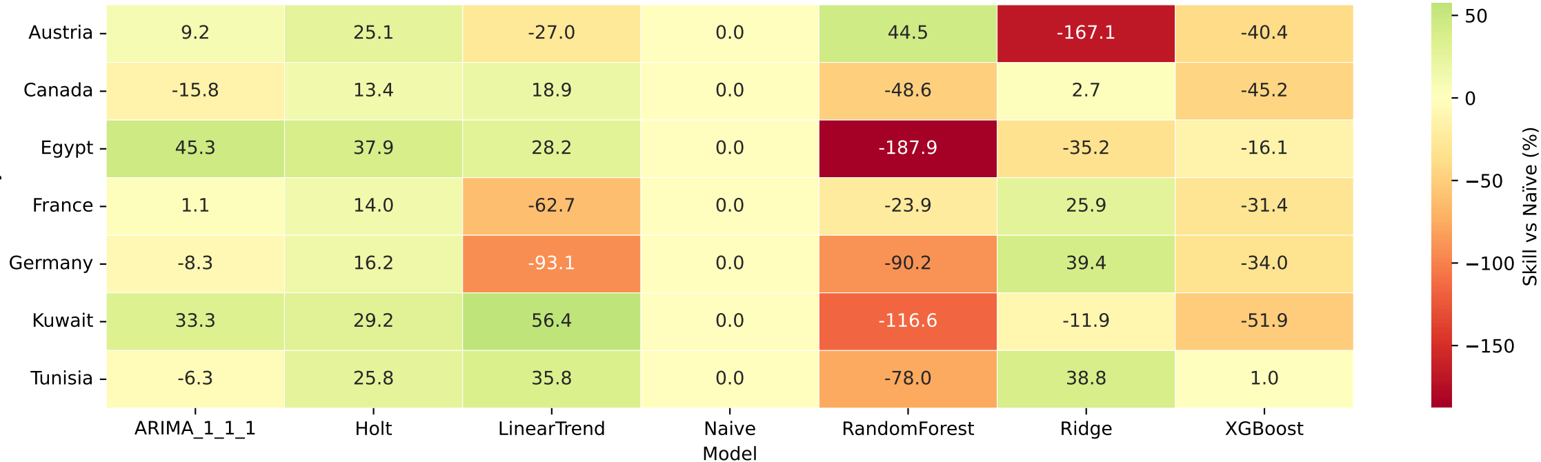
Skill Score vs Naïve Baseline (Test Set) — Higher is Better
