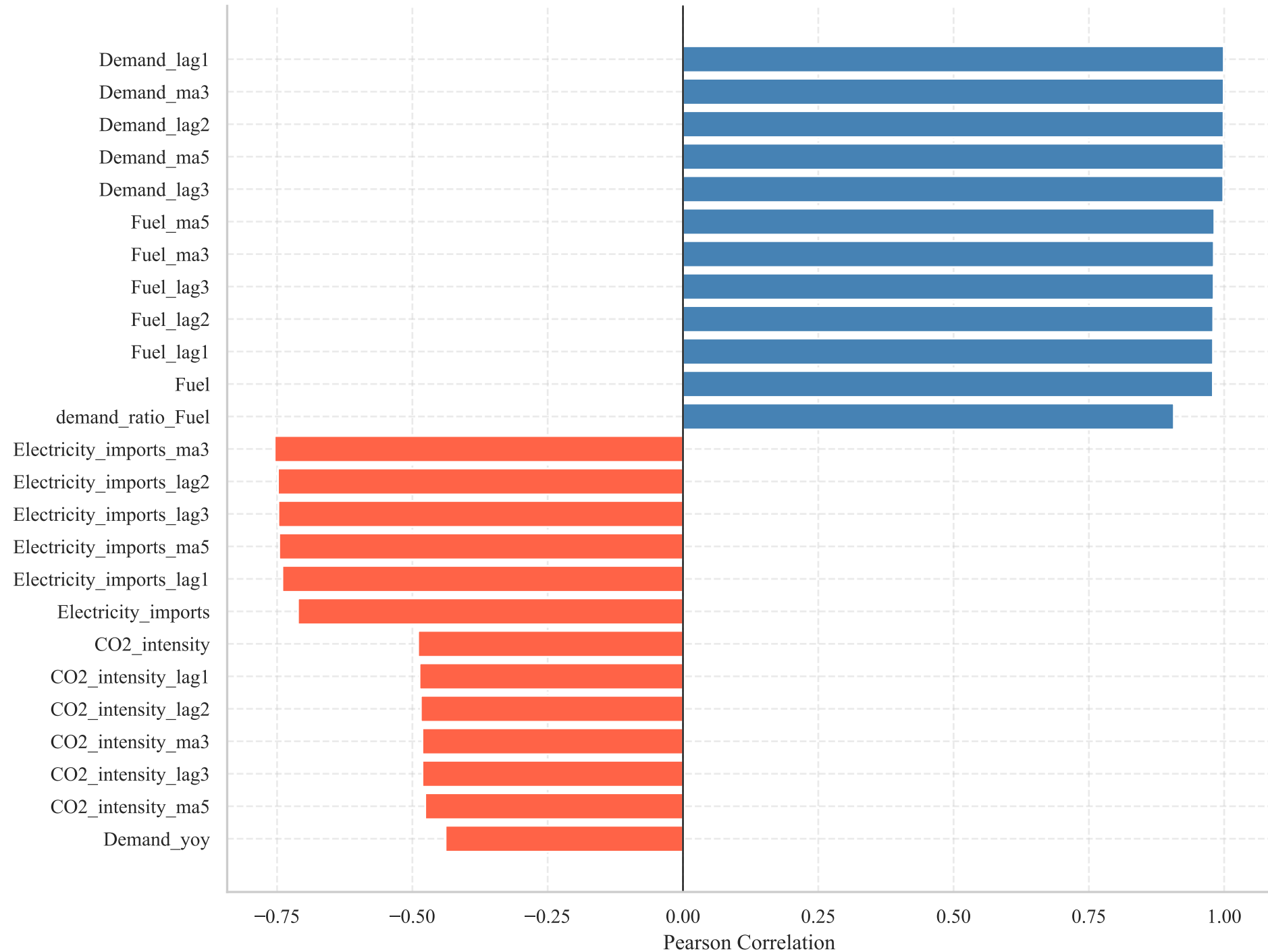
Check 5 — Top 25 Features Correlated with Demand (all engineered features)
