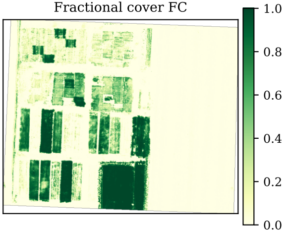
Fractional cover FC
