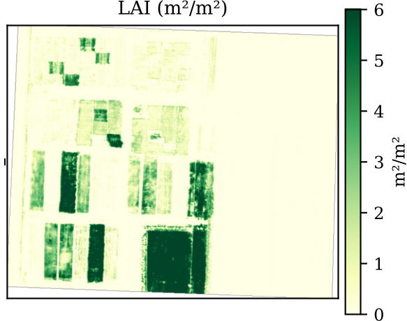
LAI ( \text{m}^2/\text{m}^2 )
