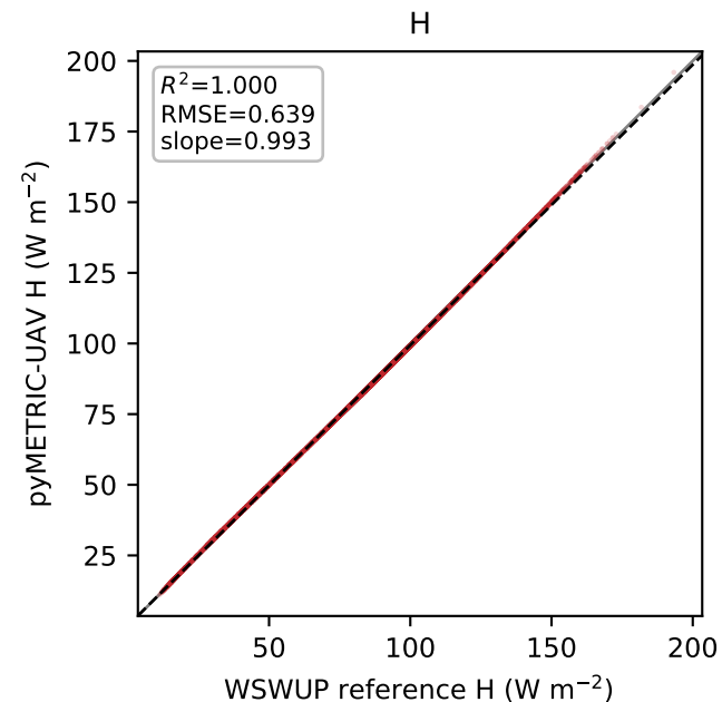
pyMETRIC-UAV vs WSWUP reference solver on the Fruita scene (identical R_n , G , T_s , anchors)
