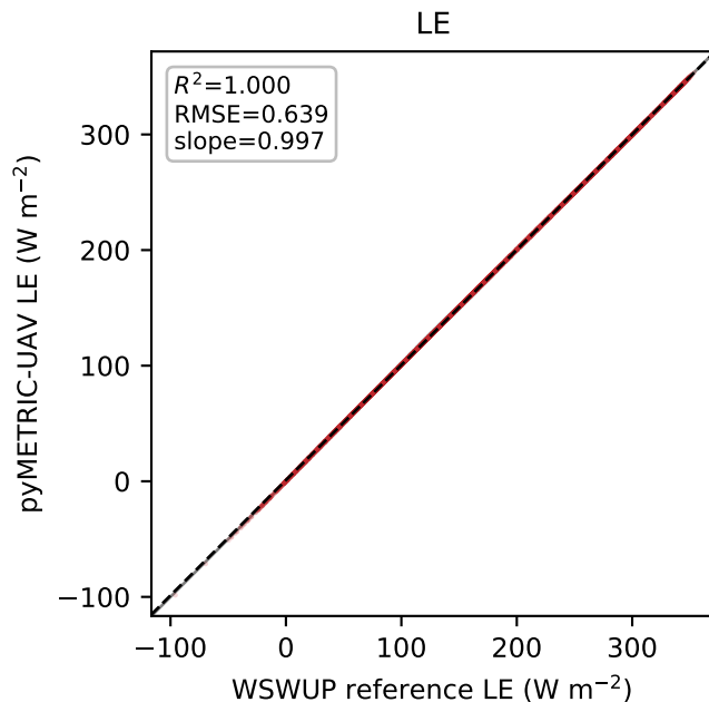
pyMETRIC-UAV vs WSWUP reference solver on the Fruita scene (identical R_n , G , T_s , anchors)
