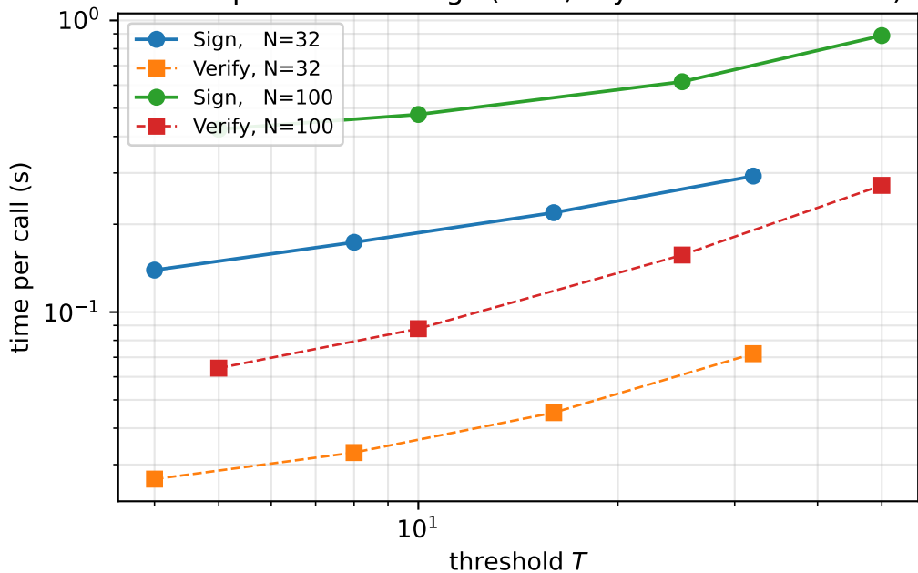
LoTRS primitive timings (Rust, rayon multi-threaded)
