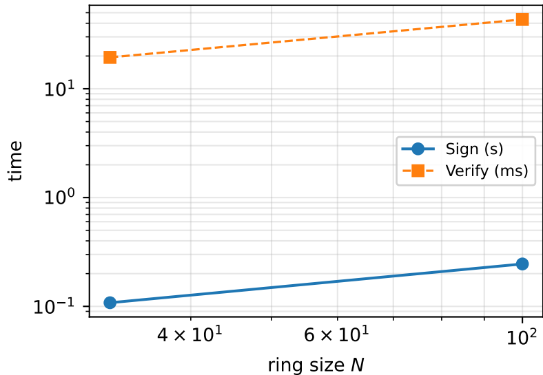
RS-alone (T=1): time vs N
