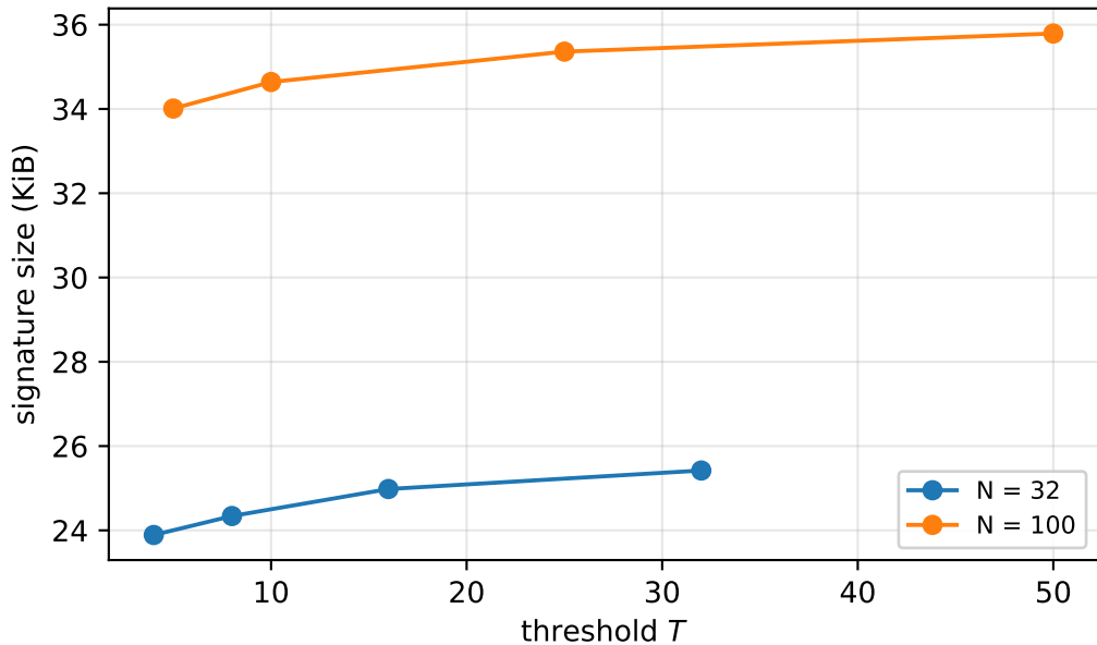
LoTRS signature size vs threshold
