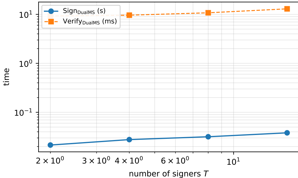
DualMS-alone (N=1): time vs T
