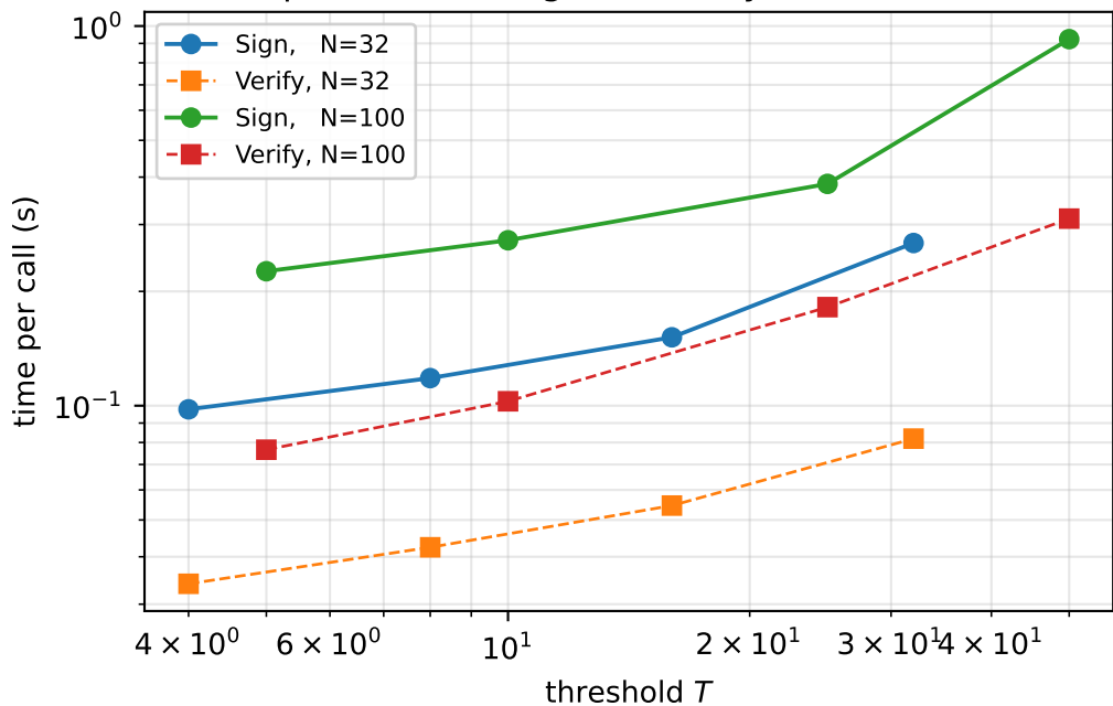
LoTRS primitive timings (Rust, rayon multi-threaded)
