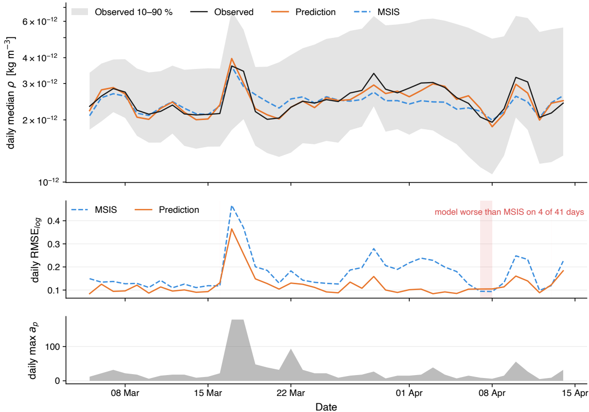
March 2015 G4 storm window — warm-start, h = 1 d ( \text{RMSE}_{\log} : MSIS 0.188 to model 0.131, -30%)
