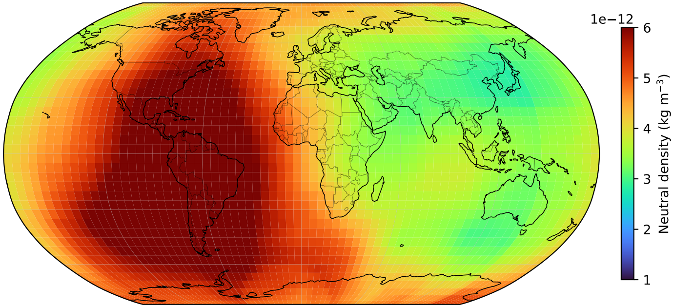
ML model
