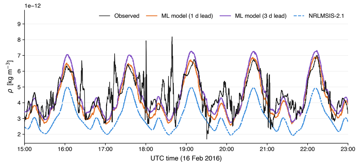
Along-track thermospheric neutral density — 16 February 2016
