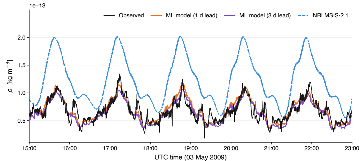
Along-track thermospheric neutral density — 03 May 2009
