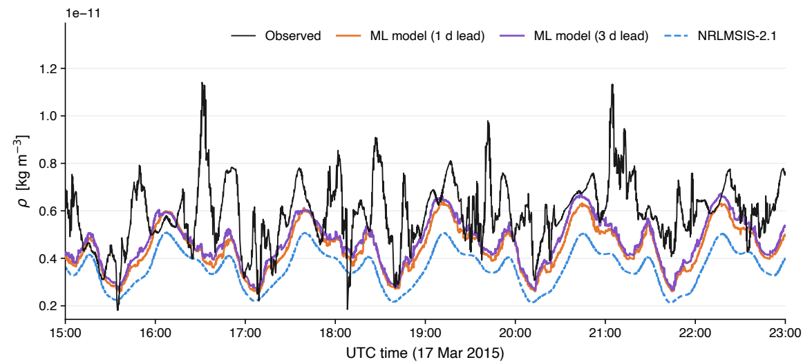
Along-track thermospheric neutral density — 17 March 2015
